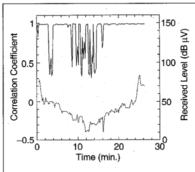
9. Comparison of received signal quality (solid line) and received level of radio wave (dashed line).
