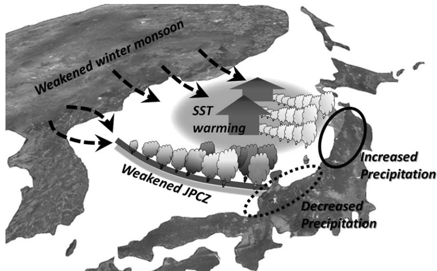
Figure 17. Schematic diagram showing the impact of SST warming on the precipitation change in JSS regions in Japan.
