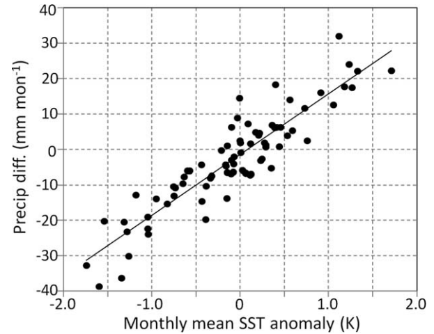
Figure 11. Scatter plot of monthly mean SST anomaly (K) during December–February over area-A (see Fig. 10) and monthly mean precipitation difference (mm month -1 ) between REAL and CLIM runs in JSS region.
