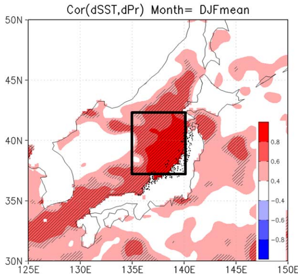
Figure 10. Distribution of correlation coefficient between DJF-mean SST anomaly and DJF precipitation difference between REAL and CLIM runs in JSS region. Solid rectangle shows the area-A (135°E–140°E, 37.5°N–42.5°N) used in Figures 11 and 12. Meteorological stations in JSS region is shown with dots. Hatched area indicates statistically significant correlation with 99% confidence level.
