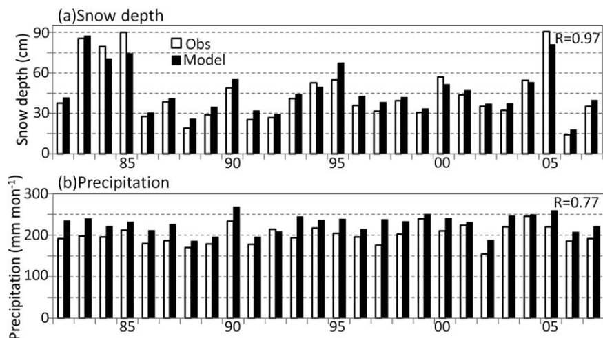
Figure 6. Interannual variation of December–January–February mean (a) snow depth (cm) and (b) precipitation (mm month -1 ) in observation (white) and REAL runs (black) for JSS region.
