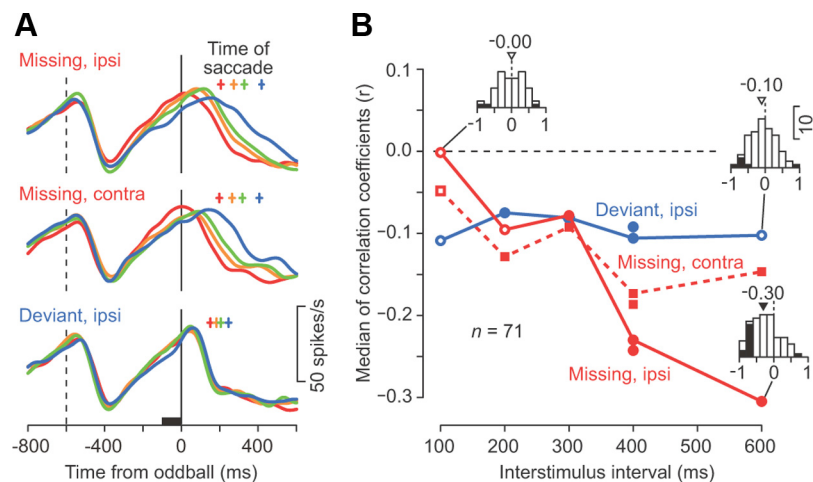
Figure 8. Correlation between neuronal activity just before the oddball and saccade latency. A , Time courses of population activity for ipsiversive missing oddball trials (top), contraversive missing oddball trials (middle), and ipsiversive deviant oddball trials (bottom) with 600 ms ISIs. For each neuron and condition, the data were divided into four groups according to saccade latencies. The population activity was computed for each of the four groups. Crosses above the traces indicate mean saccade latency for each group. B , Medians of the correlation coefficients computed between neuronal activity 100 ms before the oddball (black bar in A ) and saccade latency in individual trials. The three data points without connecting lines indicate data for trials with only visual stimuli. Filled symbols indicate data showing a significant difference from zero (Wilcoxon signed-rank test, p < 0.05 ). The inset histograms indicate the sample distributions of the correlation coefficients. The arrowhead and number on each histogram indicate the median value. Note that the negative correlation was greatest for ipsiversive saccades in the missing oddball condition and was greater for longer ISIs.
