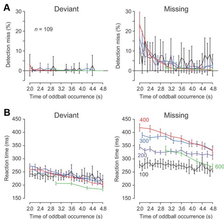
Figure 10. Behavioral data for the oddball detection task during recording sessions ( n = 109 ). A , Mean and 95% confidence intervals of the rate of detection error are plotted as a function of the time of the oddball from the first stimulus. Data from different oddball conditions (deviant and missing) are shown separately. Note that detection errors were more frequently observed with earlier occurring missing oddballs. B , Mean and 95% confidence intervals of saccade latency as a function of the time of oddball occurrence. For all panels, different colors indicate different ISIs.
