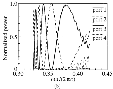
Fig. 6. Transmission spectrum of a PC waveguide coupler with two rows of rods for input pulses launched into (a) port 1 and (b) port 2.
