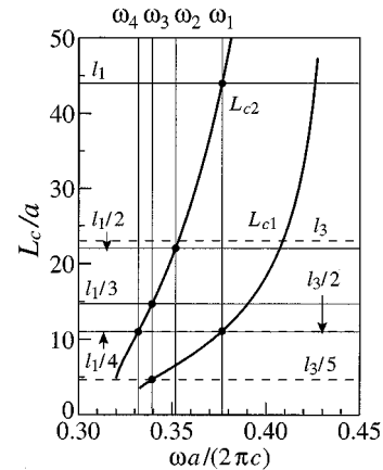
Fig. 14. Coupling lengths of PC waveguide couplers with one row and two rows of rods in the interaction region.
