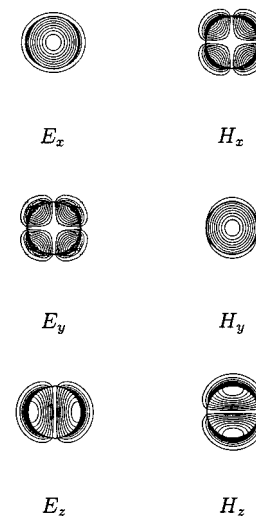
Fig. 12. Field distributions at the normalized frequency \nu = 5 for the fundamental mode in a circular waveguide.
