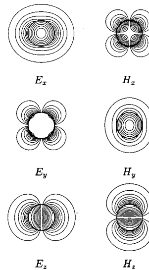
Fig. 11. Field distributions at the normalized frequency \nu = 2 for the fundamental mode in a circular waveguide.
