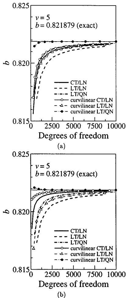
Fig. 10. Convergence of normalized propagation constant at the normalized frequency \nu = 5 for the fundamental mode in a circular waveguide calculated by using (a) the electric field and (b) the magnetic field as working variables.
