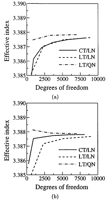
Fig. 5. Convergence of effective index for the fundamental TM-like mode in a rib waveguide calculated by using (a) the electric field and (b) the magnetic field as working variables.
