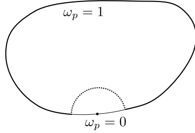
Figure 1.2: GHMD( \psi )
