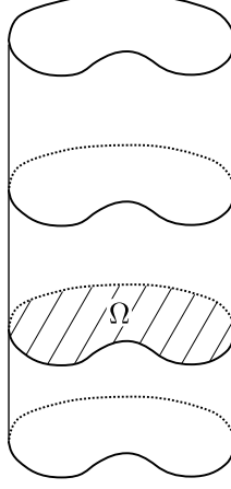
Figure 2.1: The cylinder \Omega \times \mathbb{R}
