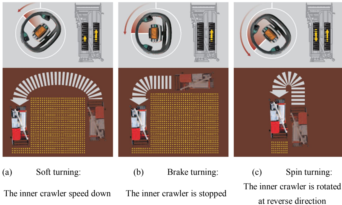
Figure 5.2 Three kinds of steering control models for the combine harvester. (AG1100).
