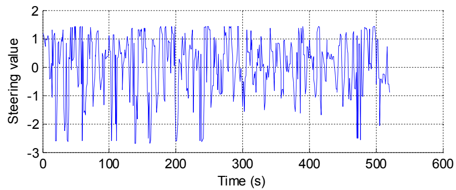
Figure 5.9 Steering value of of LS auto guidance system.
