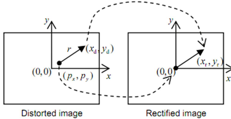
Figure 3.5 Image rectification
