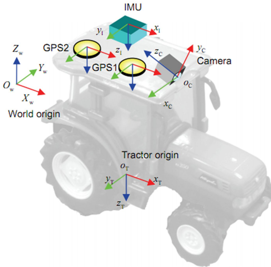
Figure 3.4 Frames of reference of the system.
