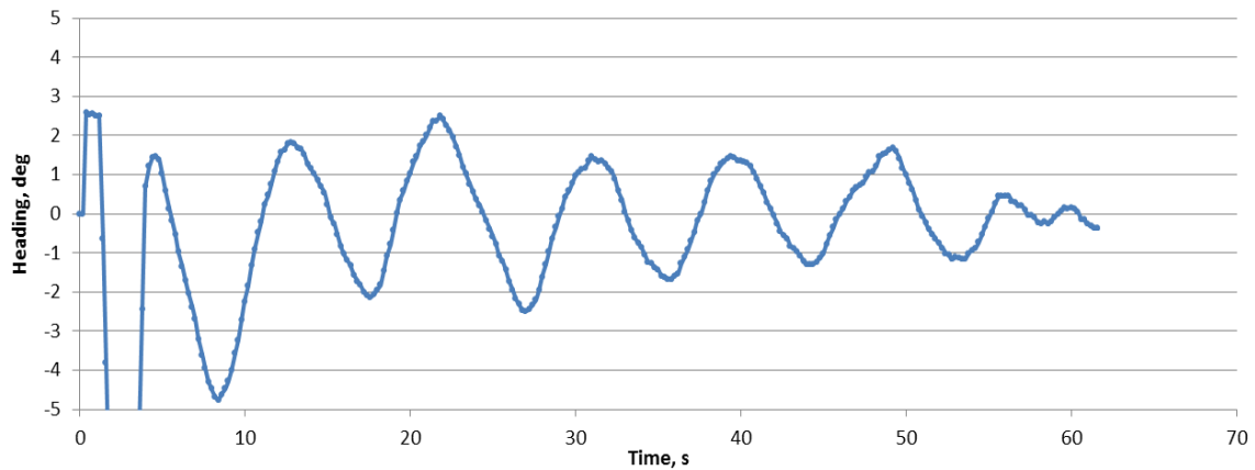
Figure 3-10 Heading error in Field Test-1
