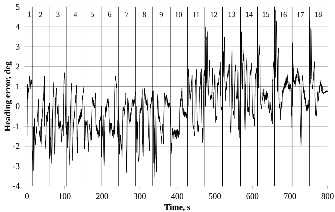
Figure 6-12 Heading error of wheat field navigation
