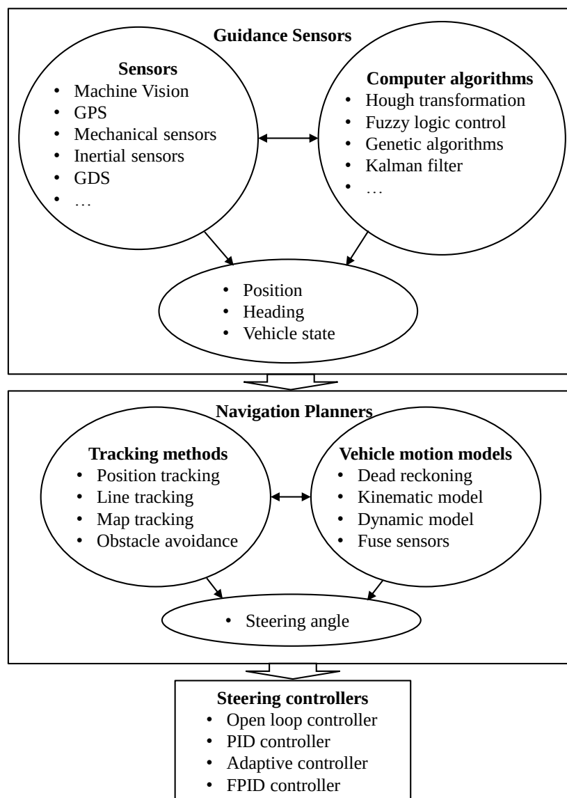
Figure 1-4 Framework of agricultural vehicle autonomous guidance system
