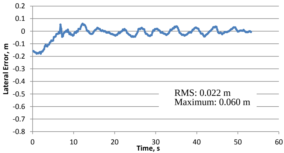
Figure 4-16 Field verification with 0.15 m of initial offset
