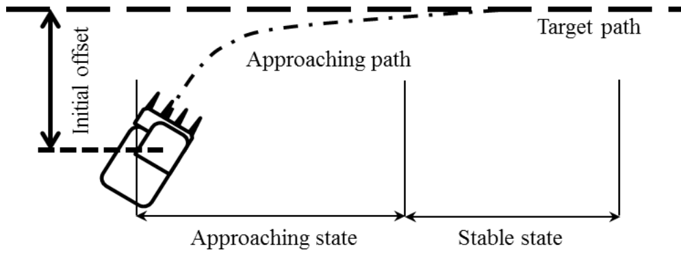
Figure 4-6 Approaching path for robot combine harvester
