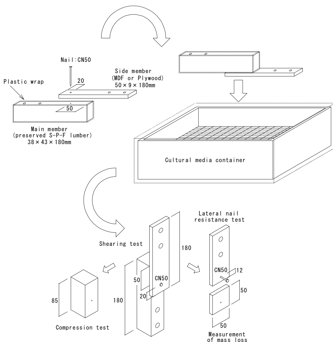
Fig. 3.1. Schematic diagram of test specimen.
