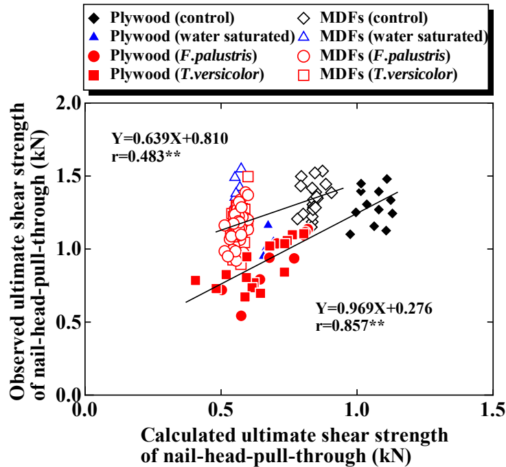
Fig. 3.13. Comparison of calculated and observed ultimate shear strength of nail-head-pull-through.
