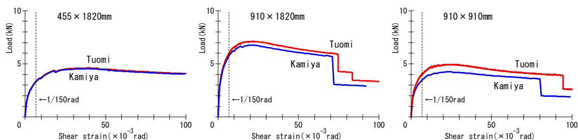
Fig. 4.12 Simulated load-strain curves of single particleboards
