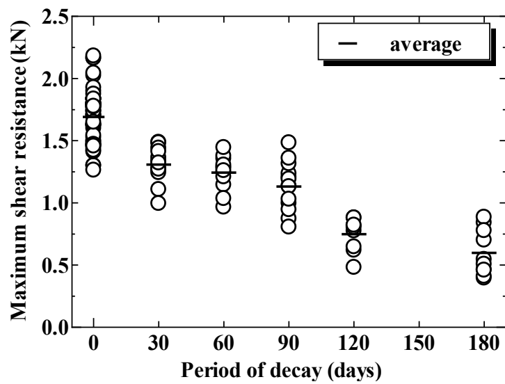
Fig. 2.12 Relationship between period of decay and maximum shear resistance of nailed timber joint with a steel plate.
