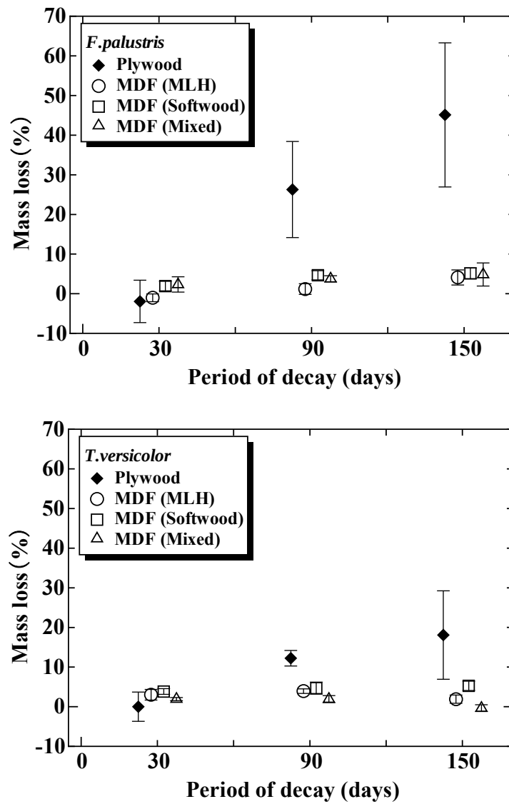
Fig. 3.3. Relationship between period of decay and mass loss. Note : Error bar : Standard deviation.
