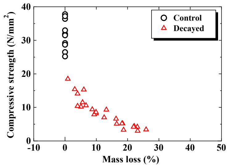
Fig. 2.9 Relationship between mass loss and compressive strength.
