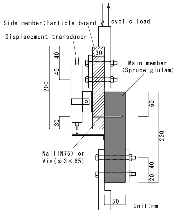
Fig. 4.6. Single shear joint test
