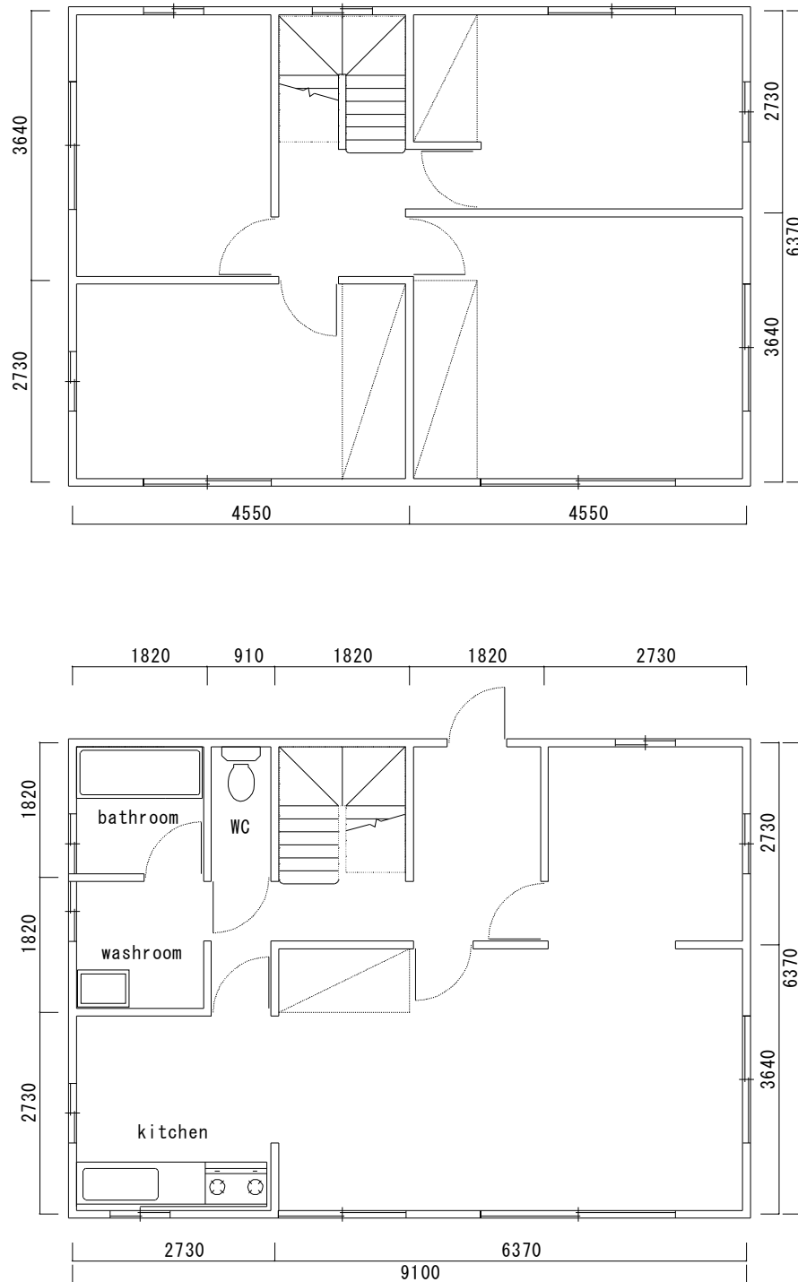
Fig. 5.1 Floor plan.
