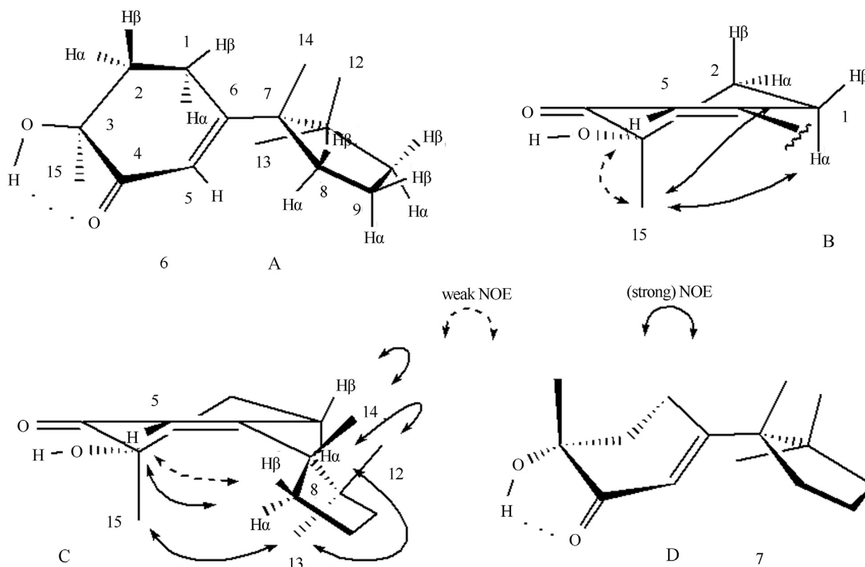
Figure 1 - A stable conformation of ( S )-(-)-cuparene-1,4-quinone (5). Important NOE correlations is shown by arrow.
