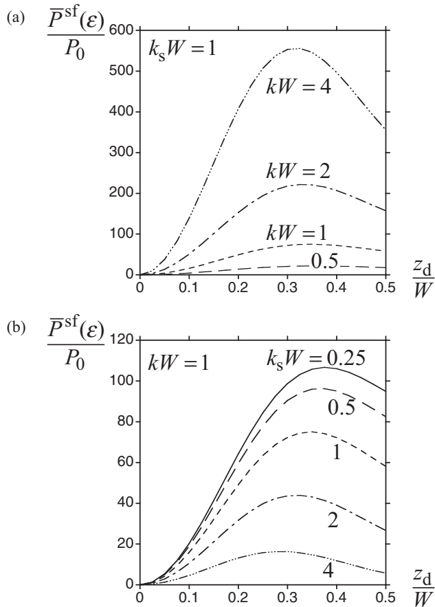
FIG. 5. Spin-flip scattering rate \bar{P}^{\text{sf}}(\varepsilon) divided by P_0 [Eq. (39)], as a function of the position of \delta doping, z_d . (a) Dependence on k = |\mathbf{k}| . (b) Dependence on k_s , the inverse of the screening length.
