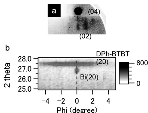
Figure 5. (a) MCP-RHEED and (b) GIXD patterns of monolayer DPh-BTBT films on 4^\circ off 1/3 ML Bi-Si(111)-( \sqrt{3} \times \sqrt{3} ) with 10 nm steps. In the MCP-RHEED pattern, two spots assigned as the (02) and (04) diffractions were observed when the electron beam was parallel to Si[112]. In the GIXD reciprocal mapping, a narrow spot assigned to the Bi(20) diffraction and wide (20) diffraction of DPh-BTBT were observed. The lattice constant derived from the (20) diffraction was a = 0.65 nm. The \phi in (b) was defined as the angle between the scattering vector of the Bragg reflection and Si[112].
