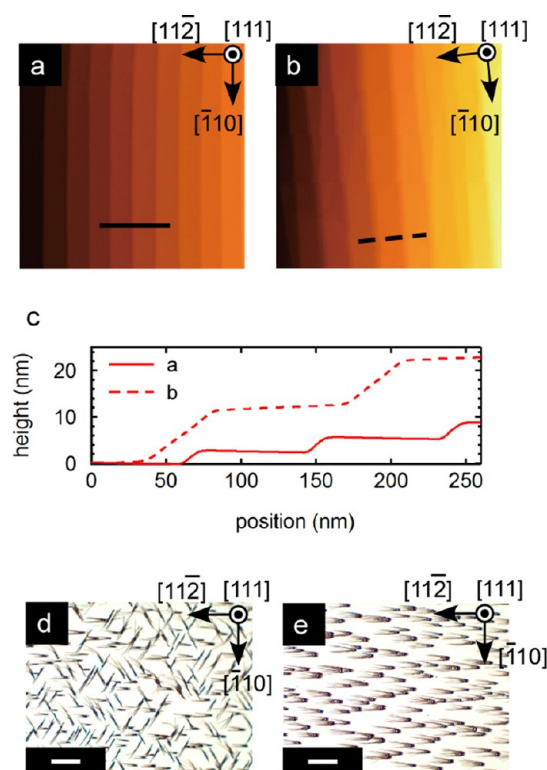
Figure 2. (a–c) AFM images and their cross section profiles of periodic bunched steps on (a) 2^\circ off and (b) 4^\circ off vicinal Si(111) surfaces inclined toward the [11\bar{2}] direction. Steps with 3 and 10 nm heights can be fabricated from 2^\circ off and 4^\circ off vicinal surface, respectively, through gradual cooling of the sample after 1260 °C flash heating. (d, e) Optical microscope image of DPh-BTBT needle crystals grown on \beta -phase Bi–Si(111)-( \sqrt{3} \times \sqrt{3} ) with (d) flat surface and (e) 10 nm steps (scale bar = 200 \mu\text{m} ). As shown in (a–c), [11\bar{2}] is the step descending direction.
