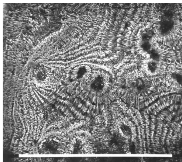
Figure 7. Microstructure of coral skeleton of Porites showing different sizes and shapes of the early mineralization zones (EMZ) and fibres. (Scale bar 100 \mu\text{m} )
