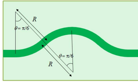
Fig. 2. Structure of the delay line. The arc-angle is fixed to \theta = \pi/6 . The path length difference is controlled by changing R .
