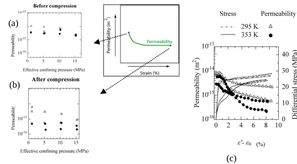
Fig. 1 Permeability of Shikotsu welded tuff.
