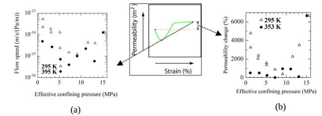
Fig. 8 Flow speed and permeability change by failure of Inada granite.
