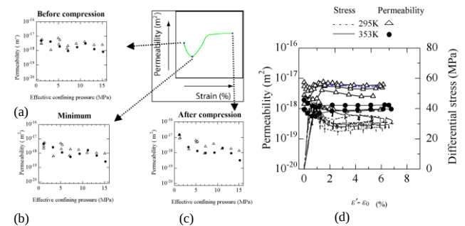
Fig. 4 Permeability of Kimachi sandstone.
