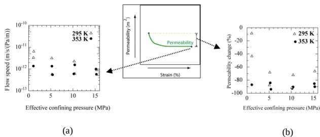
Sig. 2 Flow speed and permeability change by failure of Shikotsu welded tuff.
