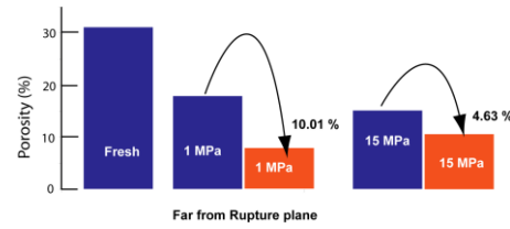
Fig. 3 Porosity of Shikotsu welded tuff after compression.
