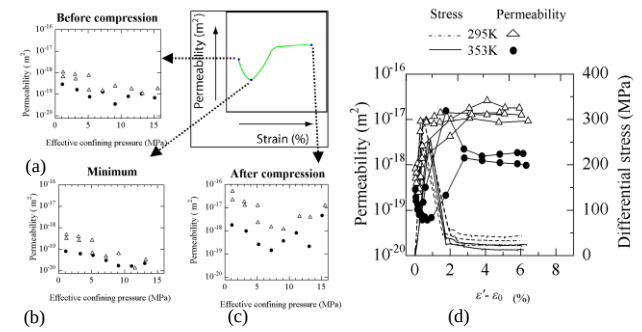
Fig. 7 Permeability of Inada granite.
