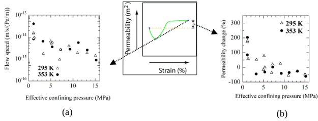
Fig. 5 Sealability and permeability change by failure of Kimachi sandstone.
