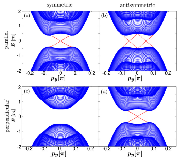
FIG. 2. (Color online) The energy spectra of the yz surface states under the symmetric Zeeman field (a) and (c) or the antisymmetric Zeeman field (b) and (d). The Zeeman field is applied in a parallel direction to the surface in (a) and (b). In (c) and (d), the Zeeman field is applied in the perpendicular direction to the surface. The momentum in the z direction is fixed at p_z = 0 in all figures.
