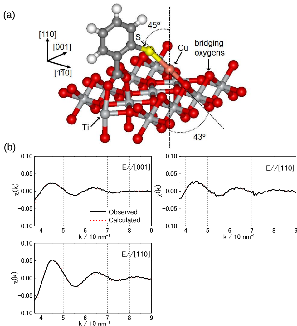
Figure 4 (a) Proposed structure of Cu/o-MBA/TiO 2 (110). (b) Cu K-edge EXAFS spectra, where the black solid and red dotted lines are the observed and calculated EXAFS oscillations, respectively. (Side and top views of the model structure and the selected atomic coordinates used for calculation are given in Supplementary Information (Figure S3 and Table S1, respectively).)
