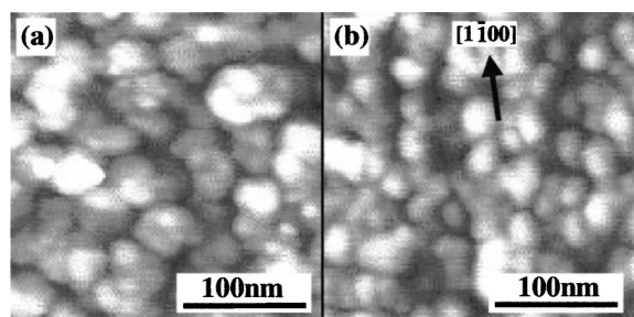
FIG. 4. AFM images of GaN coalesced islands formed on (a) the on-axis and (b) the vicinal SiC surfaces. Circular and elongated islands after coalescence are seen.
