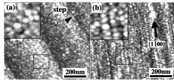
FIG. 3. AFM images of GaN nuclei formed on (a) the on-axis and (b) the vicinal SiC surfaces. Random and one-dimensionally aligned nucleation is evident on (a) the on-axis and (b) the vicinal SiC surface, respectively. Inserted figures show the magnified images of a region indicated by the square.
