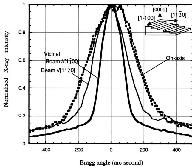
FIG. 1. X-ray rocking curves of GaN(0002) grown on the on-axis and vicinal SiC substrates. An inset figure shows the incident directions of x-ray beam on the vicinal SiC sample. Note the anisotropic feature in the vicinal sample.
