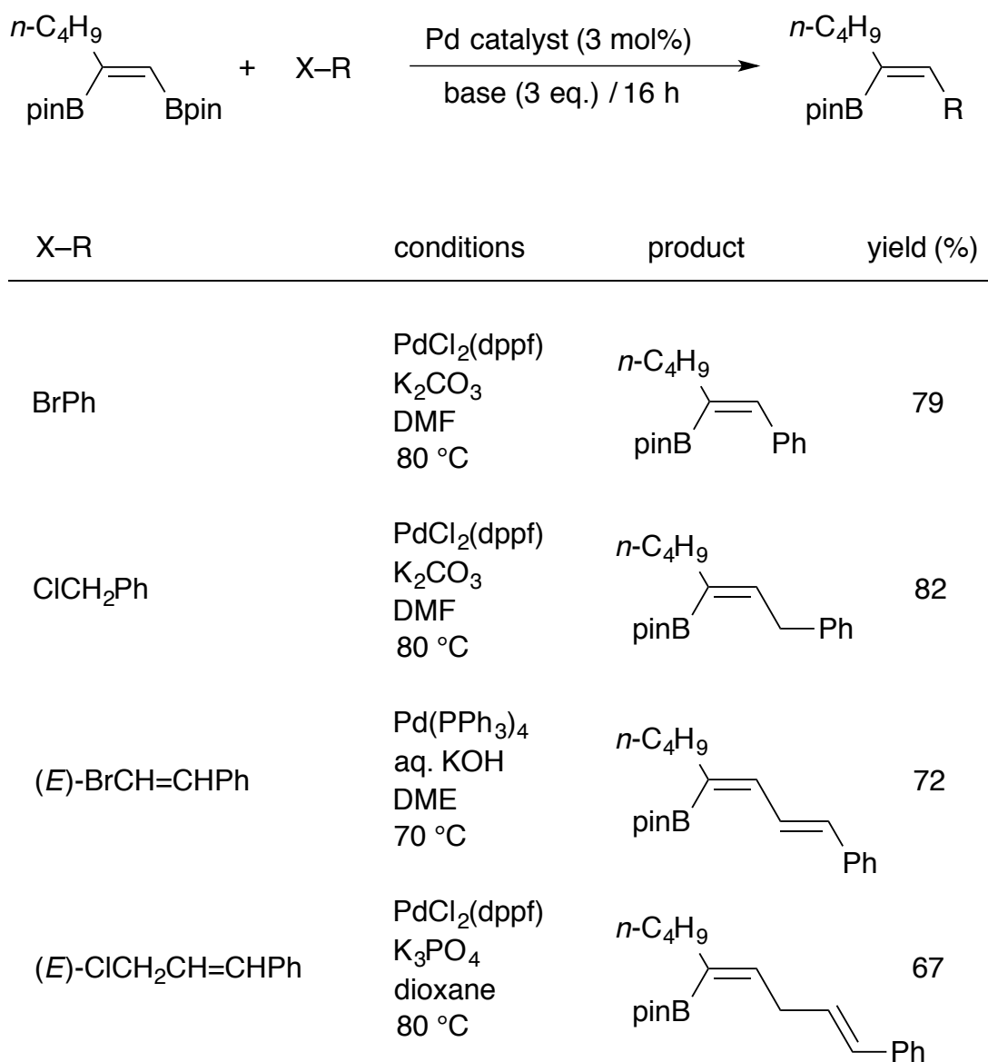
Scheme 6. Synthesis of ( E )-(1-organo-1-alkenyl)boranes
