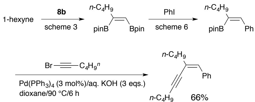
Scheme 7. Trisubstituted alkenes via a diboration-coupling sequence
