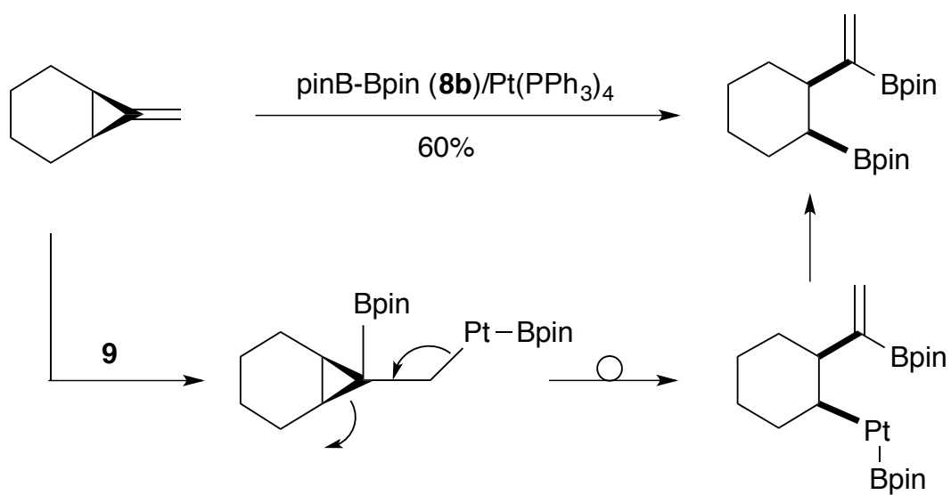
Scheme 11. Diboration of methylenecyclopropanes
