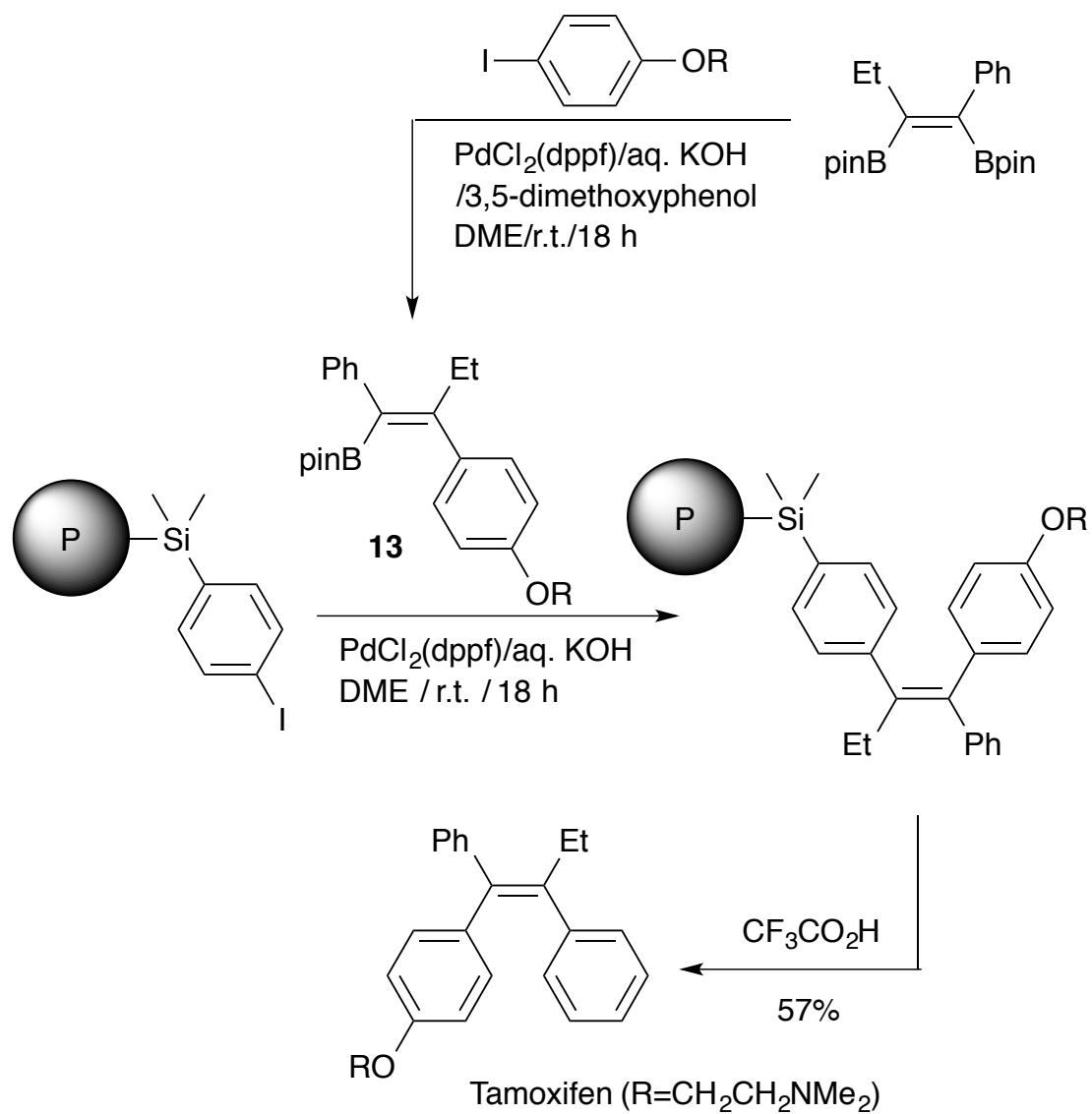
Scheme 8. Solid-phase Synthesis of tamoxifen
