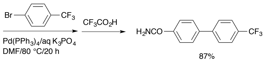
Scheme 25. Solid-phase synthesis of biaryls
