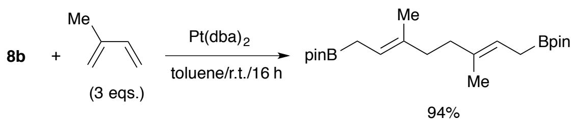
Scheme 13. 1,8-Diboration of 1,3-dienes
