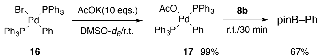
Scheme 20. (Acetoxo)palladium(II) intermediate for transmetalation
