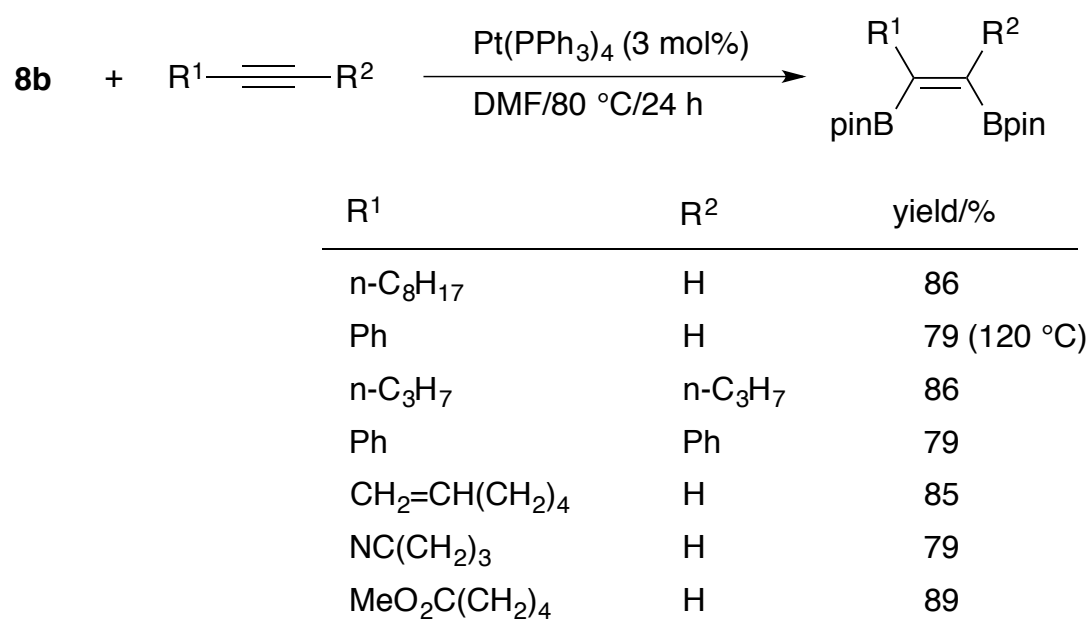
Scheme 3. Diboration of alkynes.
