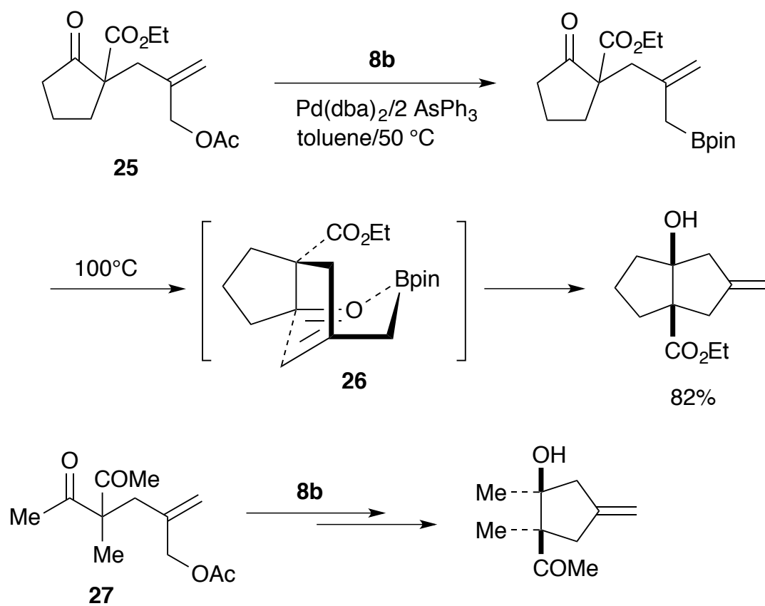
Scheme 29. Homoallyl alcohols via intramolecular allylboration
