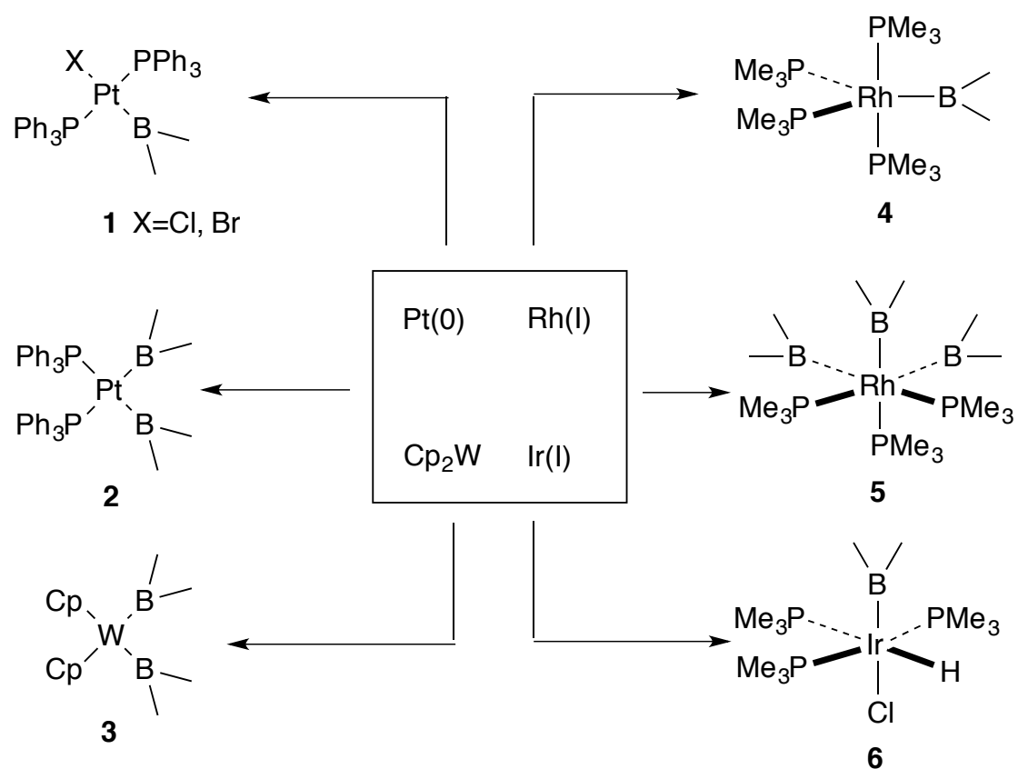
Scheme 1. Synthesis of Metal-Boryl Complexes via Oxidative Addition
