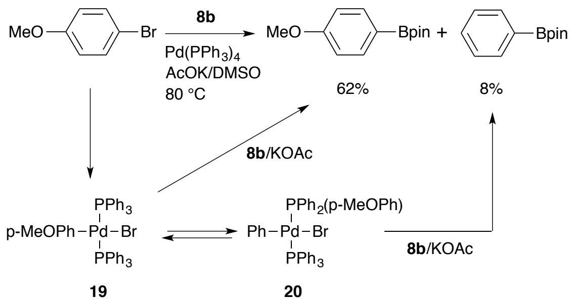
Scheme 22. Coupling with a phosphine-bound aryls
