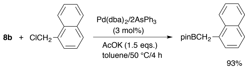
Scheme 30. Cross-coupling with benzyl chlorides
