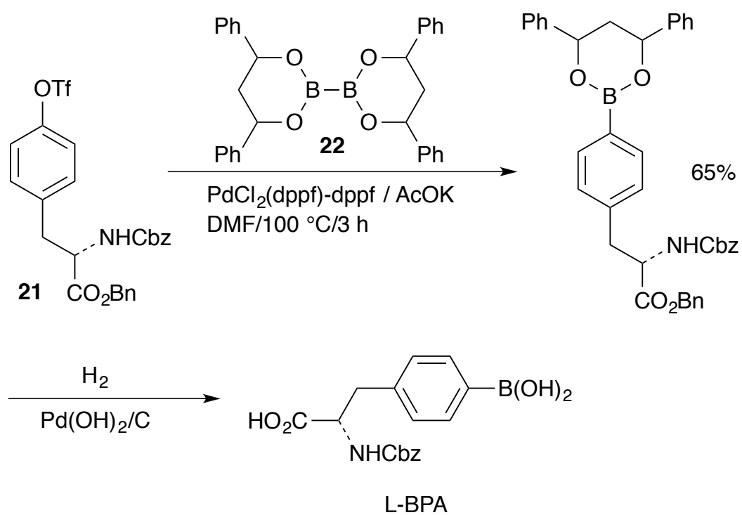
Scheme 23. Synthesis of L-BPA
