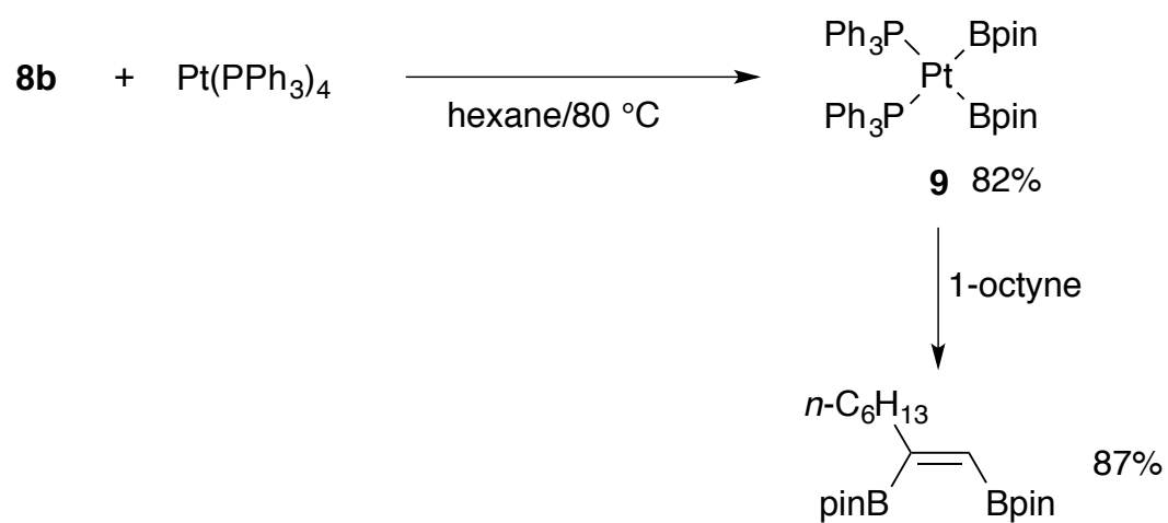
Scheme 4. Oxidative addition and insertion of diborons
