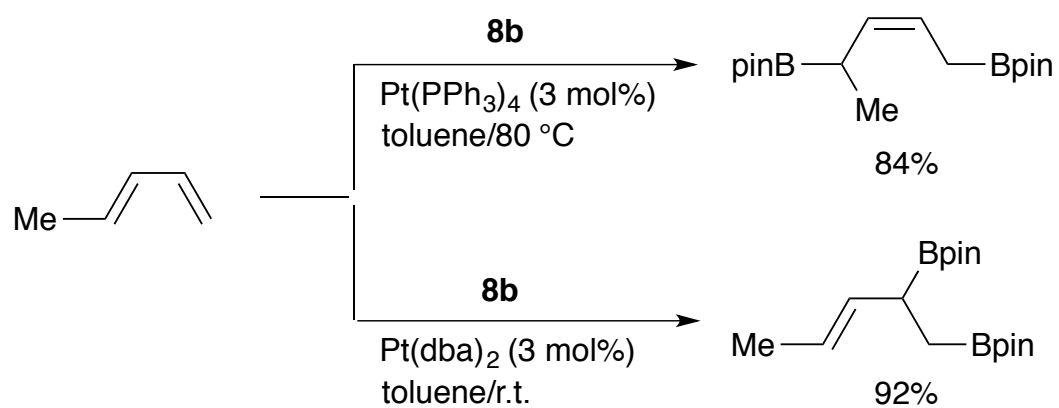
Scheme 14. 1,2- and 1,4-Diboration of 1,3-dienes
