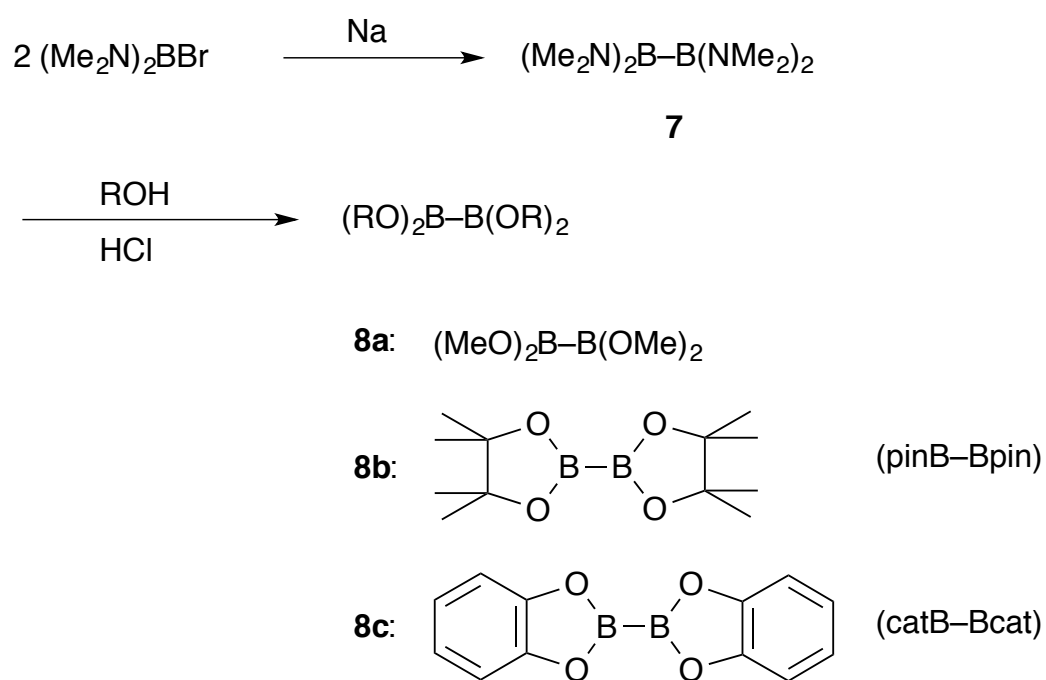
Scheme 2. Synthesis of diboron(4) compounds
