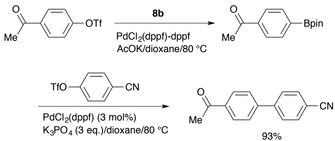
Scheme 24. One-pot synthesis of biaryls
