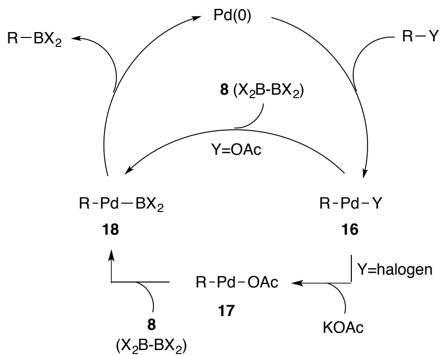
Scheme 21. Catalytic cycle for cross-coupling of diborons
