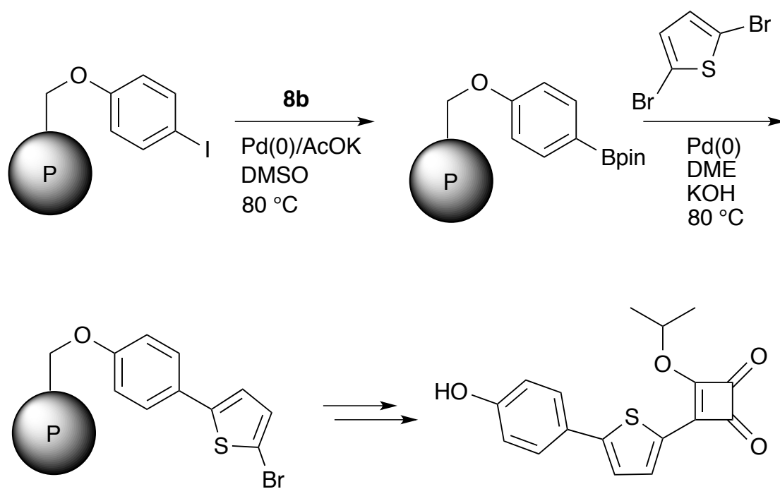
Scheme 26. Cyclobutenediones on solid support
