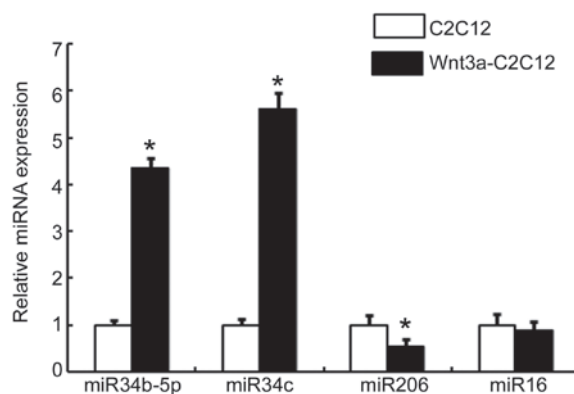
Figure 1. Regulation of miR-34b/c expression by canonical Wnt signaling. C2C12 and Wnt3a-C2C12 cells were harvested at confluence and total RNA was extracted. Expression of miR-34b-5p, miR-34c, miR-206 and miR-16 was then analyzed by qPCR and expression levels were normalized against those of sno234 RNA. *P<0.05 as determined by a t-test for paired data.
