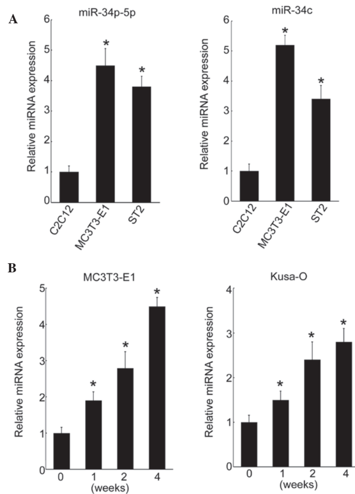
Figure 2. Expression of miR-34b/c in osteoblasts and their regulation during osteoblastic differentiation. (A) C2C12, MC3T3-E1 and ST-2 cells were harvested at confluence, and total RNA was extracted. (B) MC3T3-E1 or Kusa-O cells were cultured with 10% fetal bovine serum in \alpha -minimum essential medium containing 5 mM \beta -glycerolphosphate, 100 \mu g/ml ascorbic acid and 10^{-8} M dexamethasone for the indicated times. Total RNA was extracted and the expression levels of miR-34b-5p (A) and miR-34c (A and B) were analyzed by qPCR. Expression levels were normalized against those of sno234 RNA. * P < 0.05 compared with control, as determined by a t-test for paired data.
