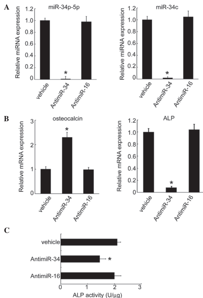
Figure 3. Effects of inhibition of miR-34b/c expression on osteocalcin and alkaline phosphatase (ALP) mRNA expression in MC3T3-E1 cells. MC3T3-E1 cells were cultured with 10% fetal bovine serum in \alpha -minimum essential medium. Following overnight incubation, the cells were transiently transfected with antimiR-34c or antimiR-16 (1 \mu M) and incubated again overnight. The culture medium was then replaced with fresh medium and the cells were cultured for a further 24 h. (A) Total RNA was extracted and the expression levels of miR-34b-5p and miR-34c was analyzed by quantitative polymerase chain reaction. Expression levels were normalized against those of sno234 RNA. (B) qPCR was performed to quantify the expression of osteocalcin and ALP mRNA. Expression levels were normalized against those of glyceraldehyde 3-phosphate mRNA. (C) The mean ALP activity of the cells. * P < 0.05 , compared with vehicle as determined by a t-test for paired data.
