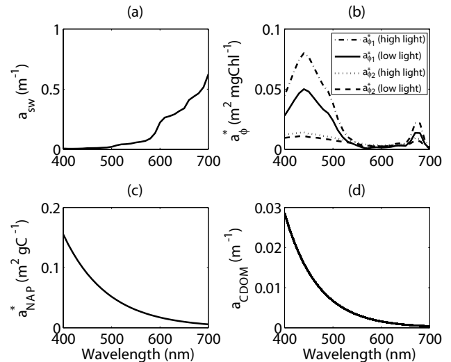
Fig. 3. Modeled (a) absorption coefficient by sea water a_{sw} ( \text{m}^{-1} ), (b) chlorophyll-specific absorption coefficients by picoplankton and diatoms ( a_{\phi1}^* and a_{\phi2}^* , respectively) ( \text{m}^2 \text{mgChl}^{-1} ), (c) carbon-specific absorption coefficient by NAP ( a_{\text{NAP}}^* ) ( \text{m}^2 \text{gC}^{-1} ), and (d) absorption coefficient by CDOM ( a_{\text{CDOM}} ) ( \text{m}^{-1} ) from 400 nm to 700 nm.
