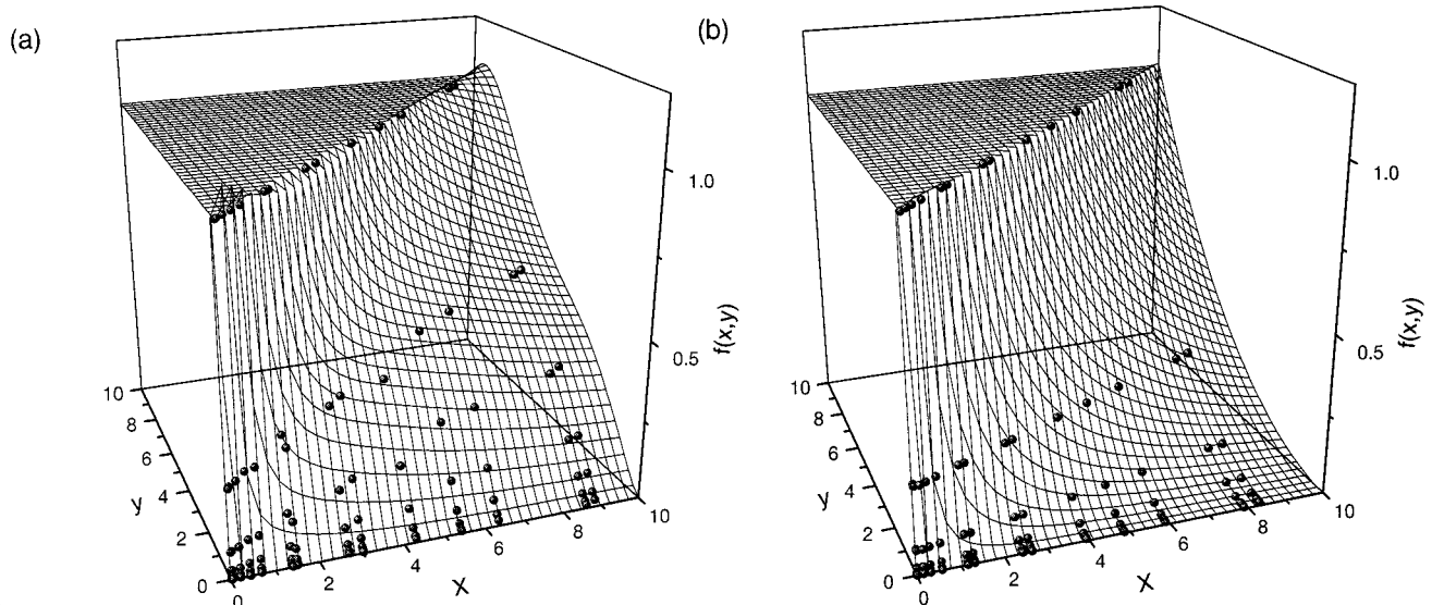
FIG. 2. Two-argument scaling functions ( q=2 ) for (a) localized and (b) extended states. Flat surfaces in the regime x < y have no meaning because the domain of f_q(x, y) is x \geq y . Calculated Z_2 in Fig. 1 are also plotted in these figures.
