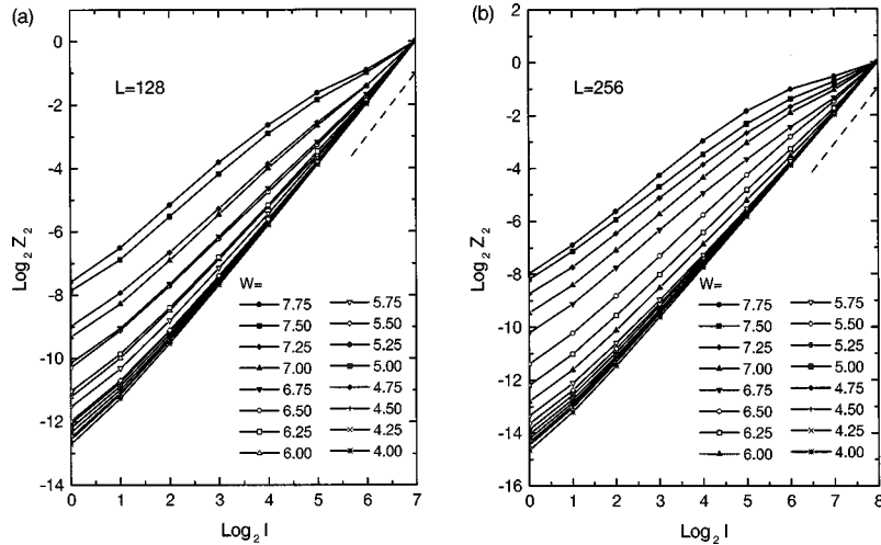
FIG. 1. Box-size dependences of quantities Z_q for q=2 . Marks correspond to different strengths of disorder. Each point has been obtained by averaging Z_2 over ten realizations of disordered potentials. (a) and (b) represent results for systems with L=128 and 256 , respectively.
