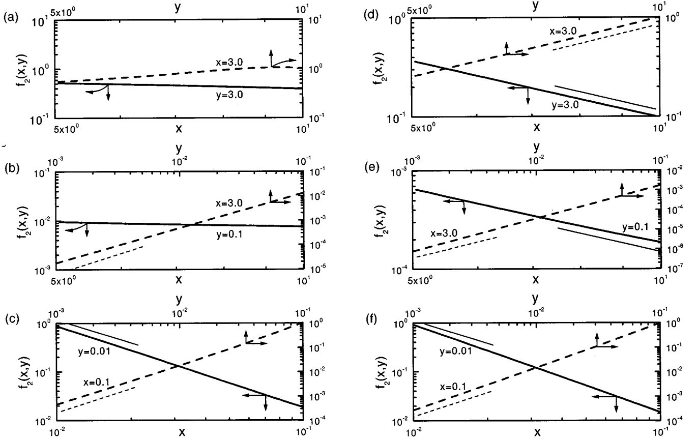
FIG. 3. Asymptotic behaviors of the calculated scaling functions. Solid and dashed lines represent the x and y dependences of the scaling functions for fixed values of y and x (indicated near lines), respectively. (a) The scaling function for localized states in the regime of x \gg 1 and y \gg 1 . (b) The scaling function for localized states in the regime of x \gg 1 and y \ll 1 . Thin dashed line indicates the slope of f_2 \propto x y^{\tau(2)} with \tau(2) = 1.62 . (c) The scaling function for localized states in the regime of x \ll 1 and y \ll 1 . Thin solid and thin dashed lines indicate slopes of f_2 \propto x^{-\tau(2)} and f_2 \propto y^{\tau(2)} with \tau(2) = 1.62 , respectively. (d) The scaling function for extended states in the regime of x \gg 1 and y \gg 1 . Thin solid and thin dashed lines indicate slopes of f_2 \propto x^{d(1-q)} and f_2 \propto y^{d(q-1)} with d=2 and q=2 , respectively. (e) The scaling function for extended states in the regime of x \gg 1 and y \ll 1 . Thin solid and thin dashed lines indicate slopes of f_2 \propto x^{d(1-q)} and f_2 \propto y^{\tau(2)} with d=2 , q=2 , and \tau(2) = 1.62 , respectively. (f) The scaling function for extended states in the regime of x \ll 1 and y \ll 1 . Thin solid and thin dashed lines indicate slopes of f_2 \propto x^{-\tau(2)} and f_2 \propto y^{\tau(2)} with \tau(2) = 1.62 , respectively.
