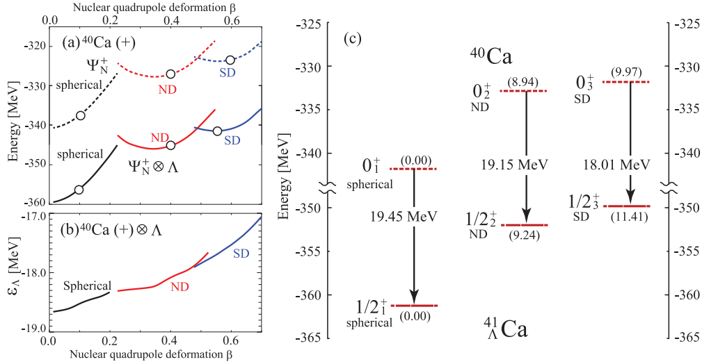
FIG. 1. (Color online) (a) Energy curves as a function of the nuclear quadrupole deformation \beta for ^{40}\text{Ca} (dotted) and ^{41}_{\Lambda}\text{Ca} (solid). Deformation parameter \gamma is optimized through the energy variation for each \beta . Open circles show the deformations \beta of the 0^+ and 1/2^+ states calculated by the GCM corresponding to the energy curves. (b) \Lambda single-particle energy defined by Eq. (13) for ^{41}_{\Lambda}\text{Ca} . (c) Calculated energies of the 0^+ states in ^{40}\text{Ca} (dotted) and 1/2^+ states in ^{41}_{\Lambda}\text{Ca} (solid). The values in parentheses are the calculated excitation energies from the ground states of ^{40}\text{Ca} and ^{41}_{\Lambda}\text{Ca} in MeV, respectively.
