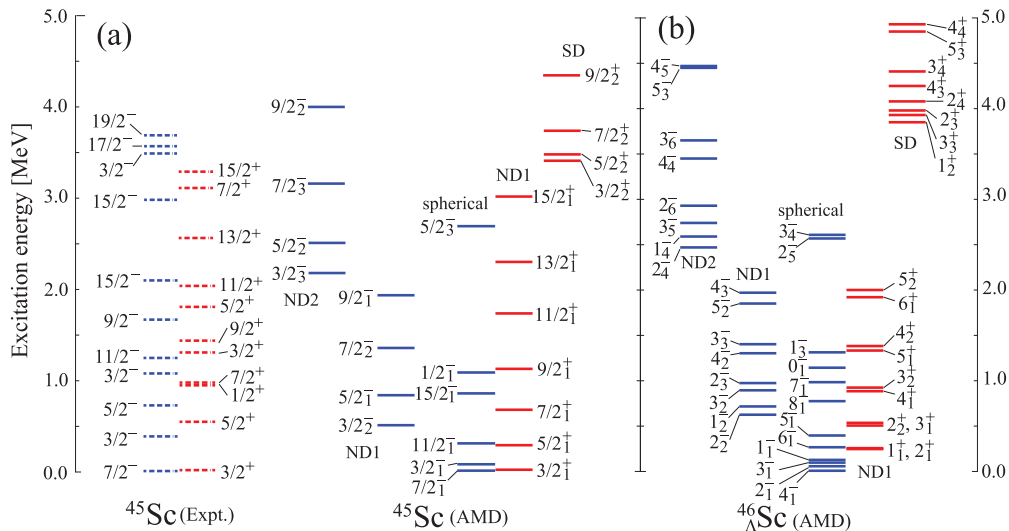
FIG. 6. (Color online) Calculated excitation spectra of ^{45}\text{Sc} and ^{46}\text{Sc} .
