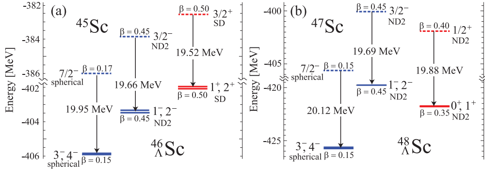
FIG. 5. (Color online) (a) Calculated energies of the ground and deformed states corresponding to the spherical, ND2, and SD minima of ^{45}\text{Sc} and ^{46}\text{Sc} shown in Figs. 2(a) and 2(b). (b) Same as panel (a) but for the spherical and ND2 minima of ^{47}\text{Sc} and ^{48}\text{Sc} shown in Figs. 2(c) and 2(d).
