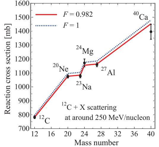
FIG. 1. (Color online) Reaction cross sections for the ^{12}\text{C} scattering on stable nuclei from A = 12 to 40. The data for ^{12}\text{C} and ^{27}\text{Al} at 250.8 MeV/nucleon are taken from Ref. [48]. The data for ^{20}\text{Ne} and ^{23}\text{Na} at 250 MeV/nucleon are deduced from the measured \sigma_1 at around 1 GeV/nucleon [49,50] with the Glauber model [17]. The data for ^{40}\text{Ca} at 240 MeV/nucleon is obtained from the measured \sigma_R at 83 MeV/nucleon [51] with the Glauber model [18]. The solid (dotted) line stands for the results of the folding-model calculations after (before) the normalization with a factor F = 0.982 .
