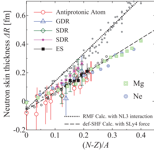
FIG. 9. (Color online) Neutron skin thickness \Delta R in Eq. (26) as a function of asymmetric parameter (N - Z)/A . The double circles and double squares denote the AMD results for the Mg and Ne isotope, respectively. The case of ^{31}\text{Ne} is not plotted here, since the nucleus has a halo structure. Neutron skin thickness is also deduced from other measurements such as antiprotonic atoms (open circles) [58], giant dipole resonance (GDR) (open triangles) [59], spin dipole resonance (SDR) (open and closed diamonds) [60,61], and proton elastic scattering (ES) (closed squares) [62,63]. The AMD results are compared with the results of relativistic mean-field (RMF) calculations with NL3 interaction (small filled dots, whose average trend is represented by the dotted line) [65], and of deformed Skyrme-HF (def-SHF) calculations with SLy4 force (small open dots, whose average trend is represented by the dashed line) [64].
