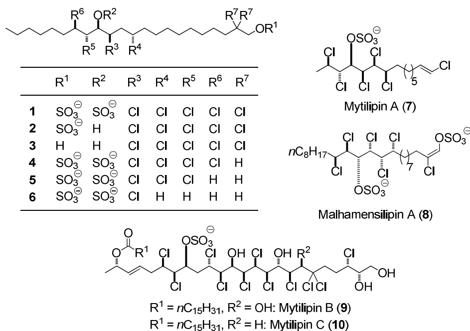
Figure 1. Chlorosulfolipids (CSLs).
