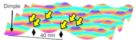
b) Three-dimensional AFM image (large-angle)
