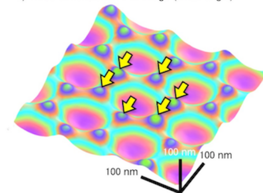
b) Three-dimensional AFM image (large-angle)
