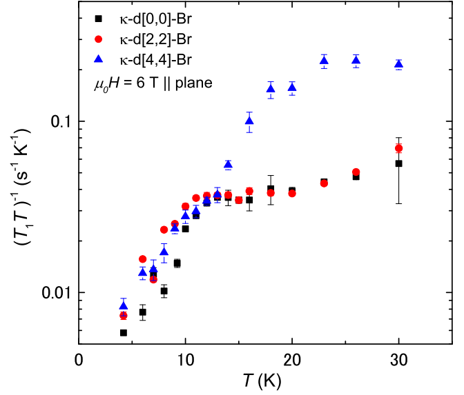
FIG. 5. (Color online) Deuteration effect on the FL state near T_c . Strong temperature dependence due to the reduction of spin term was observed in \kappa - d[4,4] -Br salt, while \kappa - d[0,0] -Br and \kappa - d[2,2] -Br salts show the FL liquid behavior below 20 K. In \kappa - d[4,4] -Br, the effects of the SC fluctuation were contaminated by the strong magnetic fluctuations near the antiferromagnetic phase transition.
