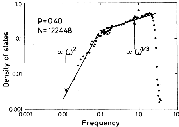
FIG. 4. The DOS per site for a 3D site-percolating network at p=0.4 formed on a 70 \times 70 \times 70 simple cubic lattice. The network size is N=122448 .
