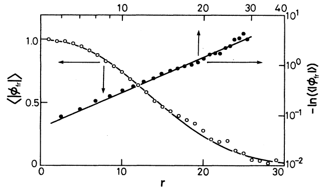
FIG. 6. The ensemble-averaged shape of the core of fractons as a function of a radial distance r (open circles) in unit of atomic spacing a=1 , and the log-log plot of r and -\ln\langle|\phi_r|\rangle (filled circles). The straight line through filled circles is drawn by the least-squares fitting, and the solid line through open circles represents the same line in a linear scale. This line indicates the exponent to be d_\phi=2.3 as well as \Lambda(\omega=0.01)=17.2 .
