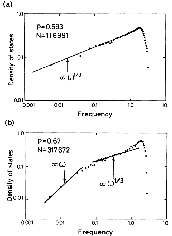
FIG. 3. The DOS's for 2D site-percolating networks at two different percolation concentrations. Filled circles indicate our numerical results and the straight lines are only a guide to the eye. (a) The DOS per site at the percolation threshold p_c ( =0.593 ). The network is formed on a 700 \times 700 square lattice and contains 116,991 atoms. (b) The DOS per site at p=0.67 formed on a 700 \times 700 square lattice. The network size is 317 672.
