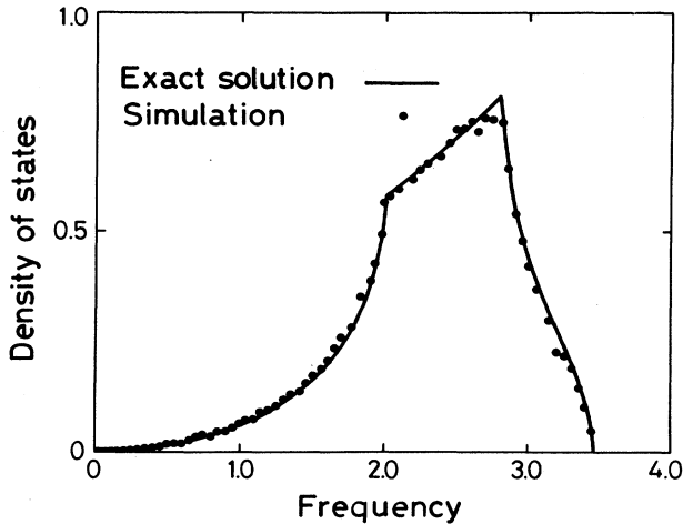
FIG. 2. The DOS for a simple cubic lattice per one atom. The solid line indicates the exact solution for the infinite system. Filled circles are our results on a 30 \times 30 \times 30 simple cubic lattice.
