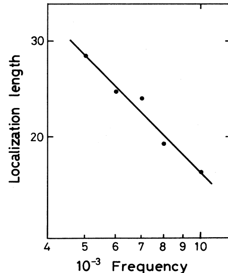
FIG. 7. Localization lengths vs frequencies of fractons plotted in a log-log scale. The straight line through filled circles is drawn by the least-squares fitting.
