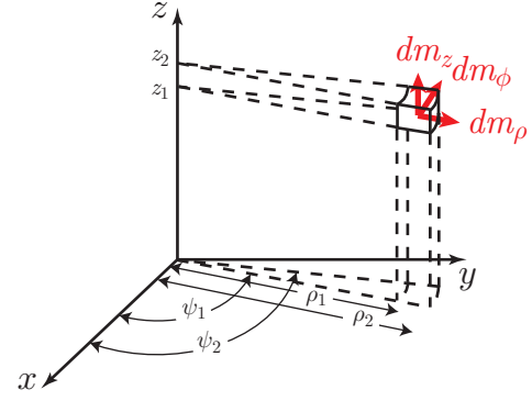
Fig. 2. Dimension of a piece of correction iron with constant magnetic moment d\mathbf{m} = (dm_\rho, dm_\phi, dm_z) in cylindrical components.
