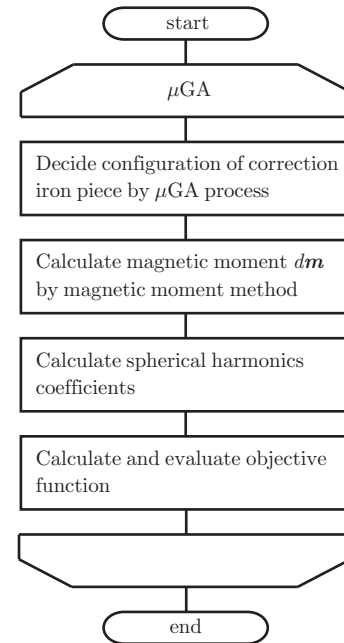
Fig. 3. Flowchart of the passive shimming computation using \mu GA.
