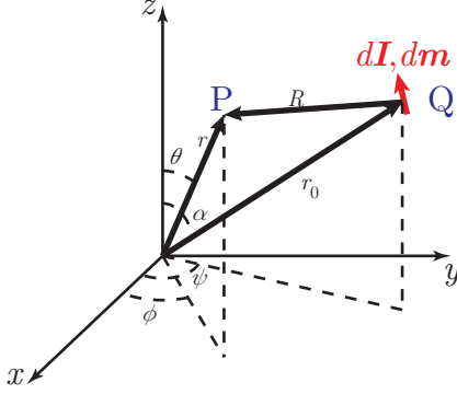
Fig. 1. Line current dI and magnetic moment d\mathbf{m} at point Q generates magnetic vector potential d\mathbf{A} and magnetic flux d\Phi at point P.
