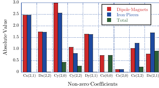
Fig. 6. The absolute value of the non-zero spherical harmonics coefficients with n = 2 .
