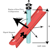
Fig. 4. Dipole magnets for magic-angle-spinning NMR. The design region of the correction iron pieces is divided into 2 (radially) \times 72 (circumferentially) \times 36 (height wise). The configuration of the correction iron pieces is optimized by the \mu GA.
