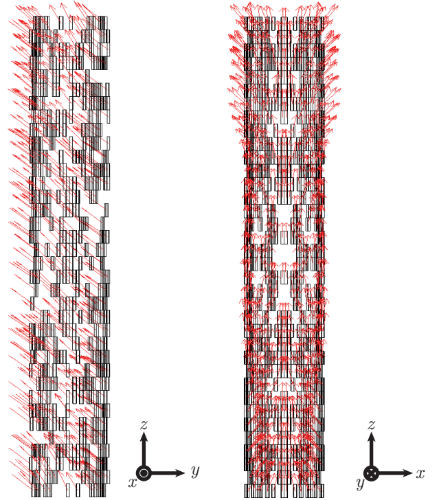
Fig. 5. The optimized configuration of the correction iron pieces with the magnetization vectors. The saturated magnetic field of the correction iron pieces is 1.2 T.
