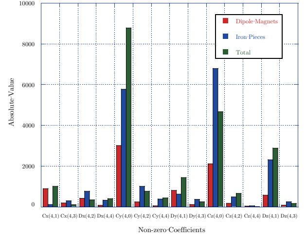
Fig. 7. The absolute value of the non-zero spherical harmonics coefficients with n = 4 .
