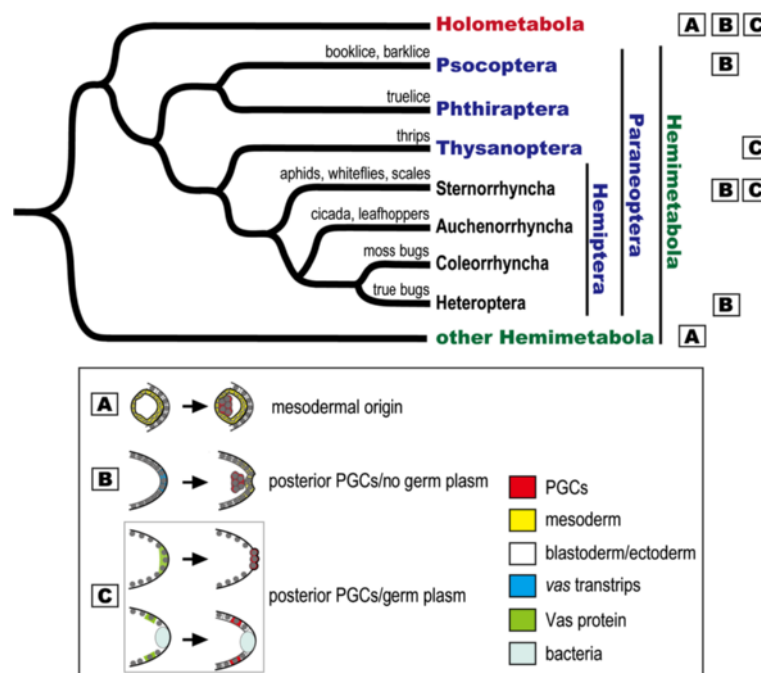
Figure 7 Phylogenetic distribution of mechanisms for germline specification within the Paraneoptera. In the phylogenetic tree we display four orders of the superorder Paraneoptera: Psocoptera (booklice, barklice), Phthiraptera (trulice), Thysanoptera (thrips), and Hemiptera (true bugs). For discussing germline specification within the Hemiptera, we present four suborders including Sternorrhyncha (aphids, whiteflies, scales), Auchenorrhyncha (cicadas, leafhoppers), Coleorrhyncha (moss bugs), and Heteroptera (true bugs). Squares A, B, and C designate mechanisms of germline specification: A, germ cells are derived from the mesoderm during mid/late embryogenesis; B, germ cells are segregated adjacent to the posterior blastoderm, which takes place after formation of the blastoderm, but a preformed germ plasm has not been identified; C, germline specification is driven by a preformed germ plasm located in the posterior pole ( Drosophila ) or slightly anterior to the posterior end (aphid) of the egg. With the exceptions of booklice ( Liposcelis divergens ; B) [62], thrips ( Haplothrips verbasci ; C) [63], and scale insects ( Pseudococcus mcdanieli , Lecanodiaspis pruinosa , and Icerya purchasi ; B) [39], where study of germline segregation was carried out with traditional microscopic approaches, mechanisms of germline specification are deduced from expression data or functional analysis of the germline marker vas/Vas . Sources for molecular data: Hemiptera: aphids ( Acyrtosiphon pisum ; C) [14], true bugs ( Oncopeltus fasciatus ; B) [36,64]; other Hemimetabola: crickets ( Gryllus bimaculatus ; A) [35]; Holometabola: honeybees ( Apis mellifera ; A) [32], the flour beetle ( Tribolium castaneum ; B) [34], fruit flies ( Drosophila melanogaster ; C) [53]. Phylogenetic relationships of the Paraneoptera are based upon Grimaldi and Engel [65]; monophyletic clades within the Hemiptera are from Wheeler et al. [66] and Cryan and Urban [67]. Abbreviation: PGCs, primordial germ cells.
