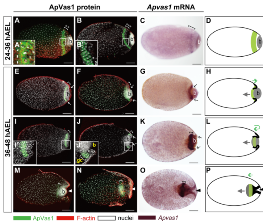
Figure 4 Expression of ApVas1/Apvas1 during germ band formation. (A, B, E, F, I, J, M, N) ApVas1 antibody staining; (C, G, K, O) Apvas1 in situ hybridization; ApVas1/Apvas1 stripes: brackets; (D, H, L, P) Schematic illustrations: migration of bacteria and ApVas1/Apvas1-positive cells are indicated with grey arrows and green double arrows, respectively; invaginating blastoderm is marked with bold lines. Anterior of egg chamber is to the left; in (M-P), anterior of the germ band is to the right. (A-D) Blastoderm embryos prior to invagination. (A') and (B') are magnifications of insets in (A) and (B), respectively. Increasing number of ApVas1-positive cells was evidenced by the expansion of stripe width (A: 2 rows; B: 3 rows; cell rows: asterisks). (C) Apvas1 mRNA was restricted to the same area as that of ApVas1 expression presented in (B). (E-H) Invagination of the posterior blastoderm. Invagination furrows marked with arrows in (F) and (G) appear more prominent than those in (E). Posterior boundary of the ApVas1/Apvas1 stripe moved to encounter the anterior border of the bacteria. (I-L) Co-migration of bacteria and the ApVas1/Apvas1 stripe into the yolk. Embryos in (I) and (J) belong to the same preparation but are shown at different focal planes: (I), cortex; (J), interior. (I') and (J') are magnifications of insets in (I) and (J), respectively. (K) Apvas1 expression. (L) ApVas1/Apvas1 stripe first reaches to the posteriormost end of the egg and then migrate back inside the yolk. After that, they follow the migration of bacteria. (M-P) Immersion of the ApVas1/Apvas1 stripe into the yolk during anatrepsis. (M) Continuous invagination of the posterior blastoderm pushed bacteria and ApVas1 stripes toward the central region of the egg chamber. (O, N) Cells expressing ApVas1/Apvas1 and bacteria were located at the posterior region of the germ band. Abbreviation: b, bacteria; gc, germ cells. Scale bars: 100 \mu m.
