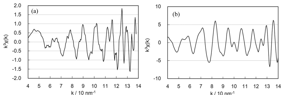
Figure 10. (a) Pt K-edge and (b) Pt L III -edge k^3 -weighted XAFS oscillations for Pt/C at 0.4 V vs RHE after background subtraction and normalization of the spectrum in Figure 9.
