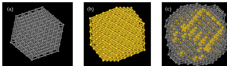
Figure 12. Estimated structures of (a) Pt cuboctahedron, (b) Au cuboctahedron, and (c) Pt/Au core-shell particle.
