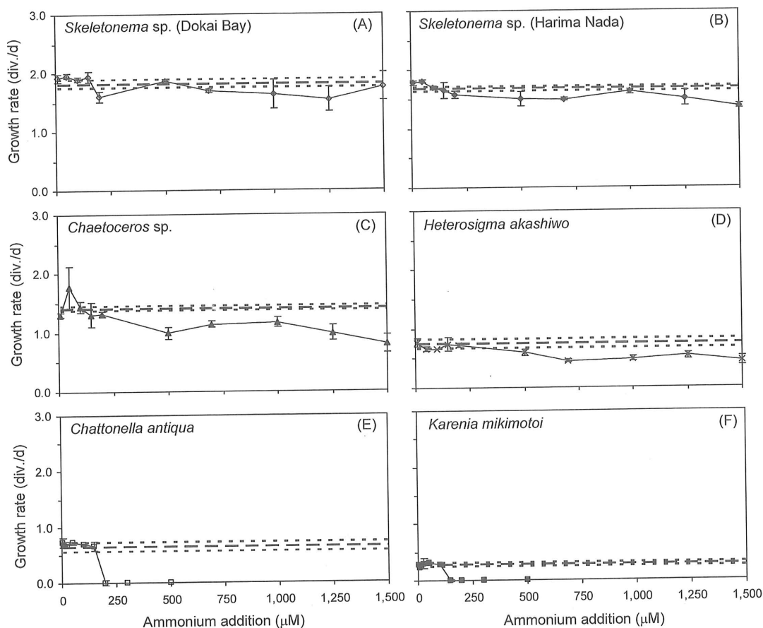
Fig. 2. Growth rates ( \mu , divisions day -1 ) of Skeletonema sp. isolated from Dokai Bay (A) and Harima Nada, Seto Inland Sea (B), Chaetoceros sp. (C), Heterosigma akashiwo (D), Chattonella antiqua (E) and Karenia mikimotoi (F) exposed to various ammonium addition. Vertical bars are standard deviations (S.D.) of replicate samples. Longer dashed lines indicate the growth rate of the control treatment (no \text{NH}_4^+ addition) and shorter dashed lines indicate \pm S.D.
