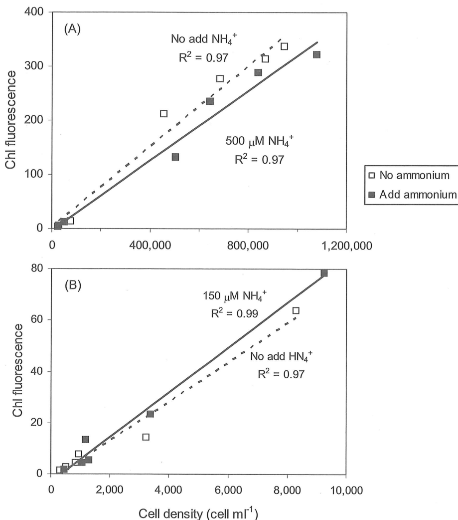
Fig. 1. Correlation between chlorophyll fluorescence and phytoplankton cell density of Skeletonema sp. (A) and Chattonella antiqua (B) under different ammonium concentrations.
