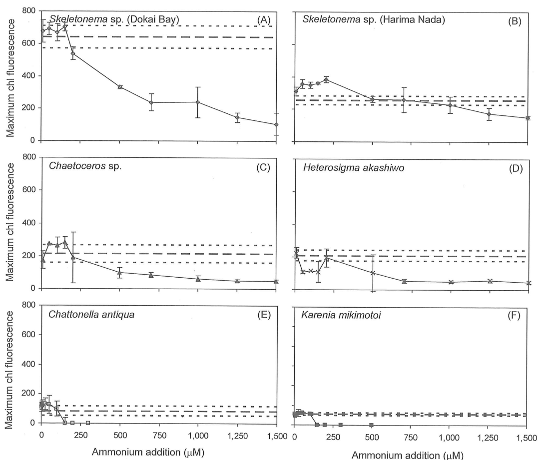
Fig. 3. Maximum chlorophyll fluorescence of Skeletonema sp. isolated from Dokai Bay (A) and Harima Nada, Seto Inland Sea (B), Chaetoceros sp. (C), Heterosigma akashiwo (D), Chattonella antiqua (E) and Karenia mikimotoi (F) exposed to various ammonium addition. Vertical bars are standard deviations of replicate samples. Longer dashed lines indicate the maximum chlorophyll fluorescence of the control treatment (no \text{NH}_4^+ addition) and shorter dashed lines indicate \pm S.D.
