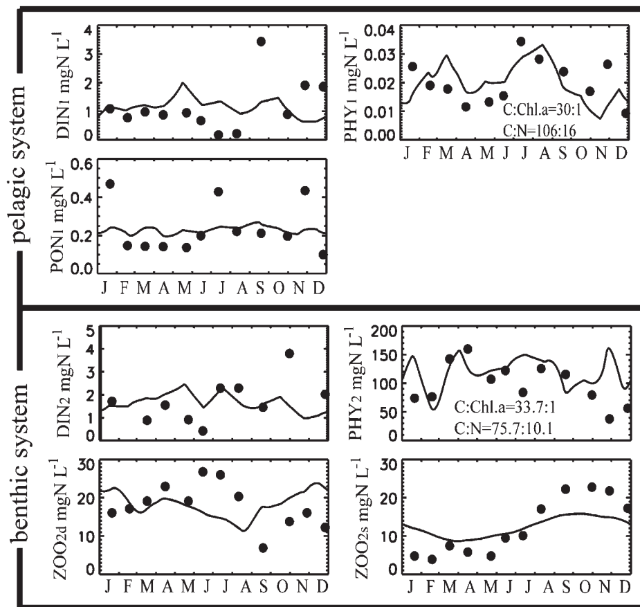
Fig. 5. Seasonal variations in calculated (full line) and observed (dot) values of \text{DIN}_1 , \text{PHY}_1 , \text{PON}_1 , \text{DIN}_2 , \text{PHY}_2 , \text{ZOO}_{2d} , and \text{ZOO}_{2s} in the tidal flat of the Seto Inland Sea.
