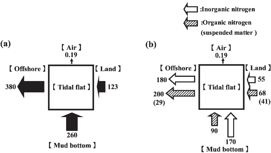
Fig. 10. Annually averaged values of nitrogen budget (a) and inorganic and organic nitrogen budgets (b) in the present case with the suspension feeder.
