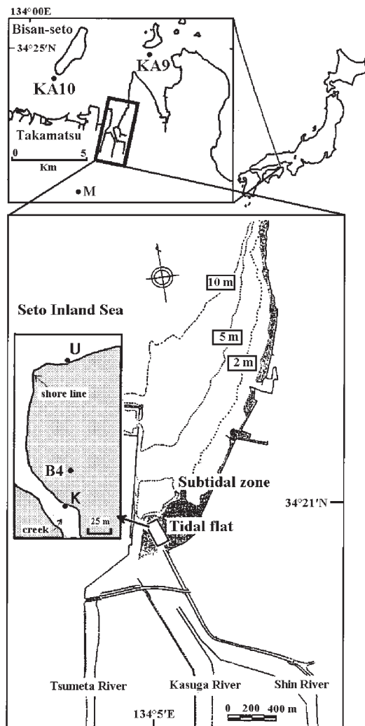
Fig. 1. Study area and location of sampling stations. Stn. B4: station for Box 2 and Box 3 in sediment, Stn. U and Stn. K: stations for Box 1 in water column, Stn. KA9 and Stn. KA10: stations for Box 4 in Bisan-seto, M: Takamatsu Meteorological Observatory.
