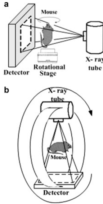
Fig. 2.2. Scanning geometry: (a) rotation bed, (b) rotation gantry. (Figure reprinted from [2.5]).
