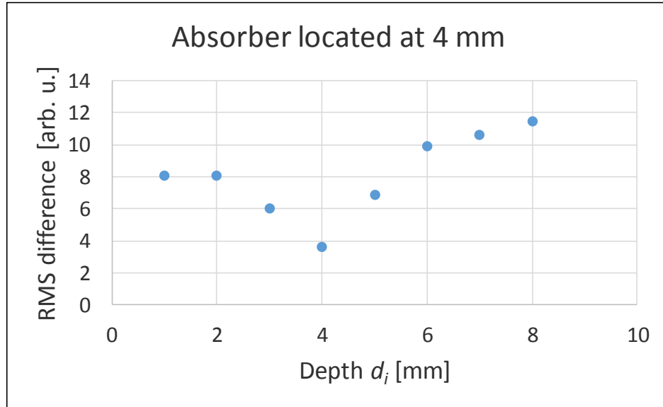
Fig. 8.10. Estimation depth of absorber ( d_t = 4.00 mm).
