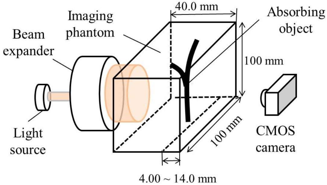
Fig. 4.21. Experimental setup for transillumination imaging: d = 4.00\text{--}14.0\text{ mm} .
