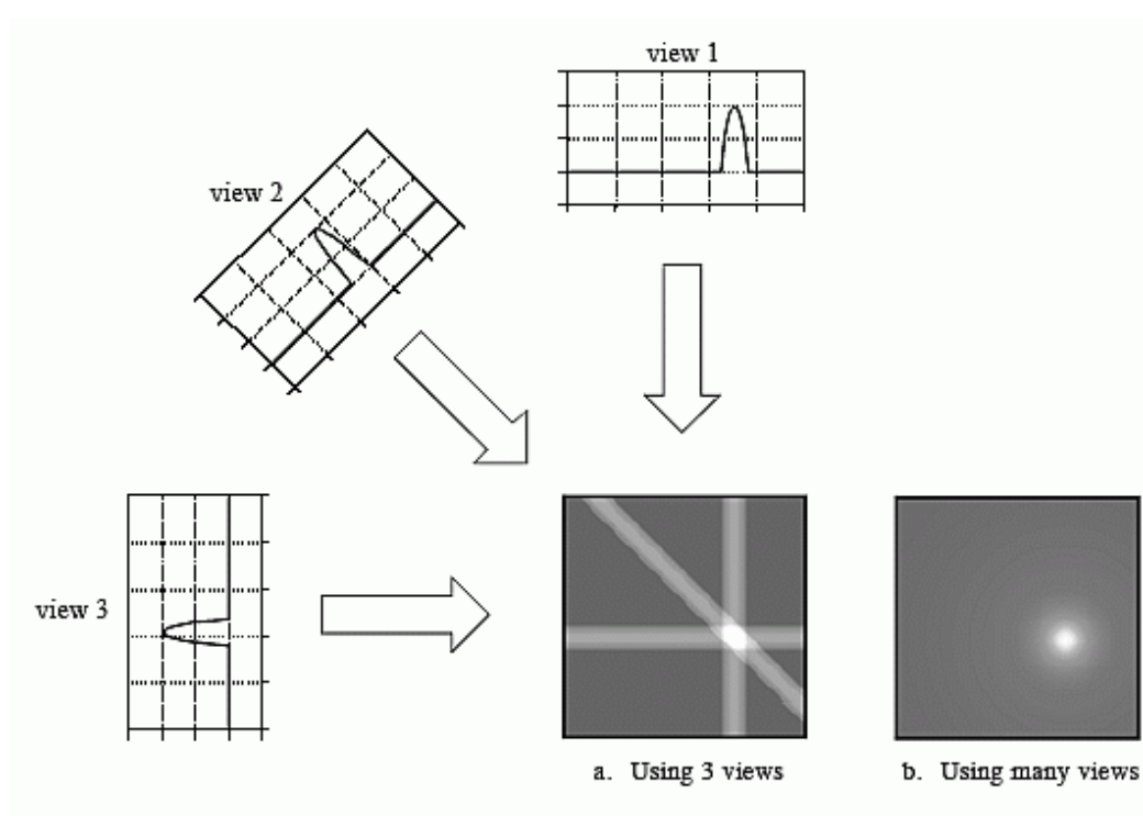
Fig. 3.2. Example of simple back-projection. Back-projection reconstructs an image by taking each view and smearing it along the path it was originally acquired. The resulting image is a blurry version of the correct image. (Figure reprinted from [3.7]).
