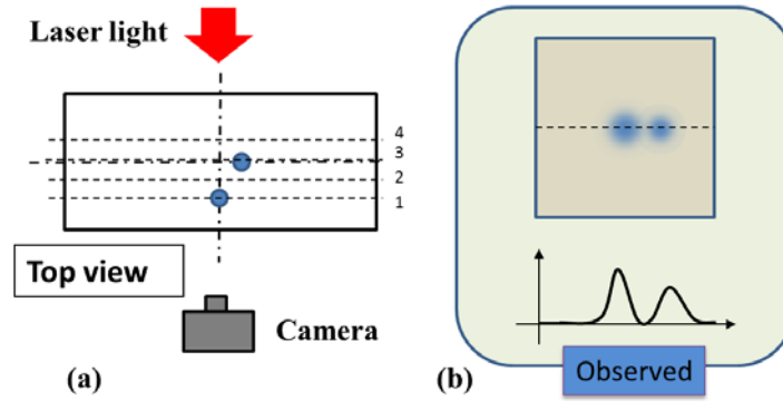
Fig. 6.1. Two absorbing objects in turbid medium: (a) top view of observing condition, (b) observed transillumination image and absorption profile along the dashed line.
