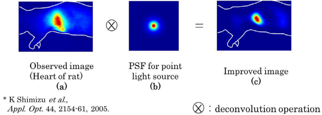
Fig. 3.10. Example of the improvement of transcutaneous fluorescence image using depth-dependent PSF: (a) observed image, (b) depth-dependent PSF, (c) improved image. \otimes denotes the deconvolution operation. (Figure adapted from [3.22]).
