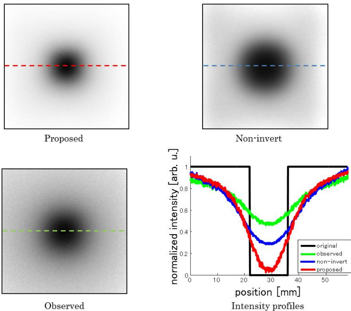
Fig. 4.17. Result with transillumination image of the absorber at d = 6.00 mm. The intensity profiles show the distribution of light intensity along the dashed lines.
