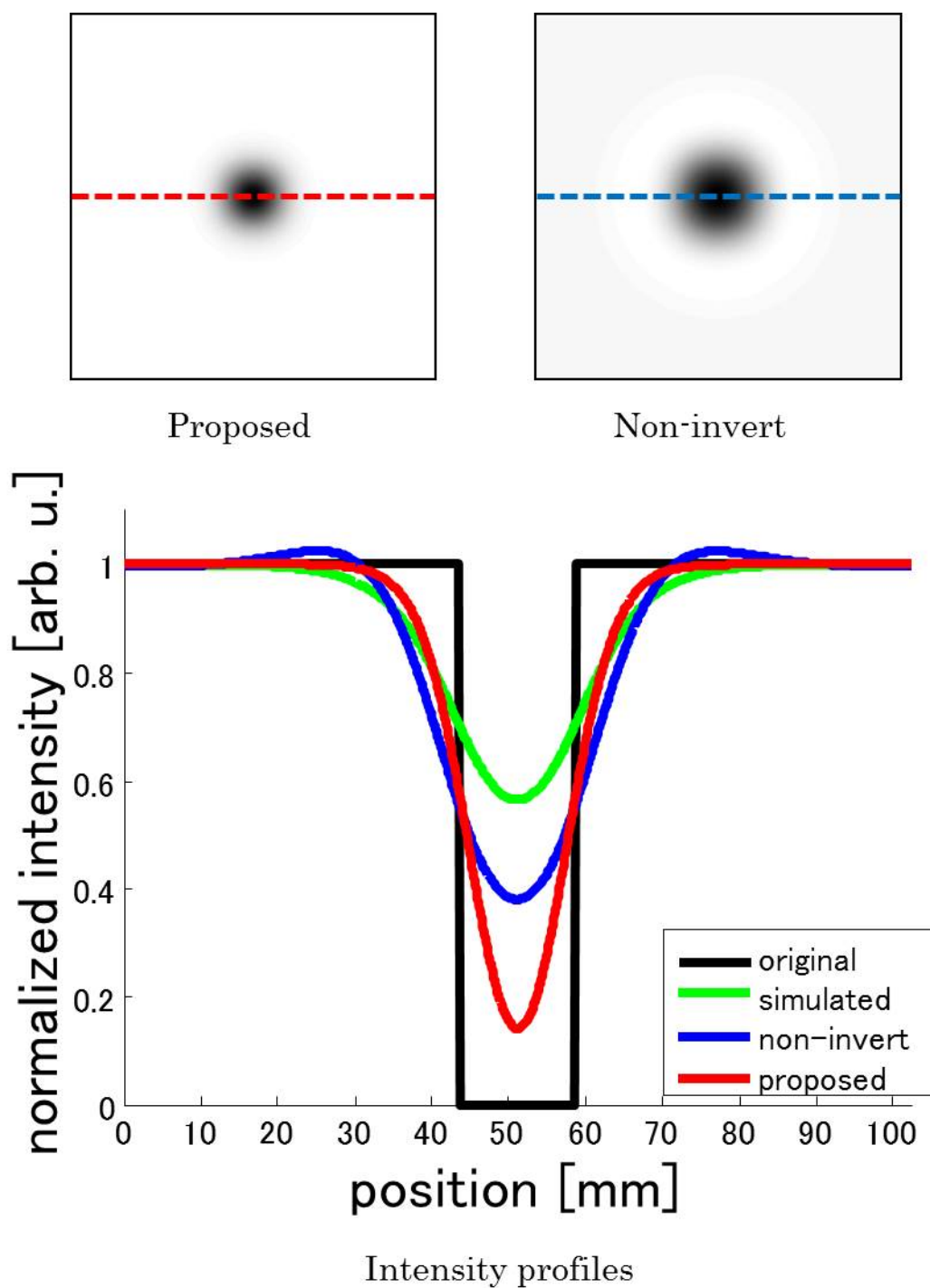
Fig. 4.13. Result of the scattering suppression technique using light-source PSF at depth d = 10 mm.
