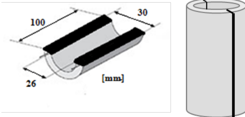
Fig. 7.3. Light trap structure.
