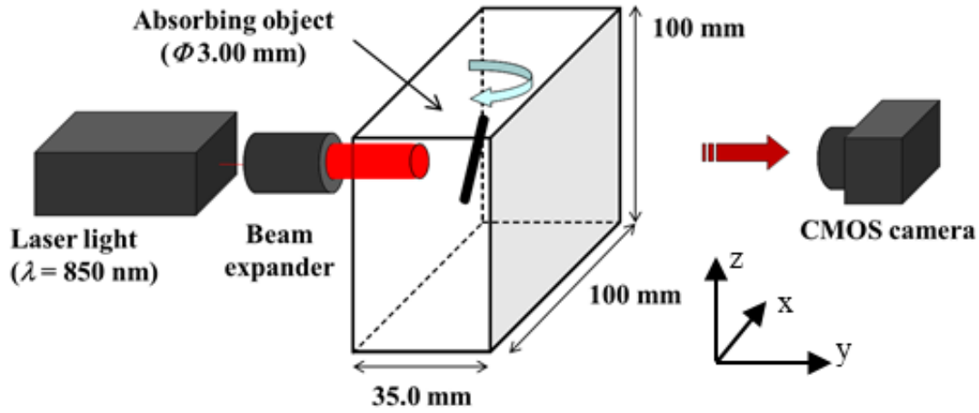
Fig. 5.1. Experimental setup.
