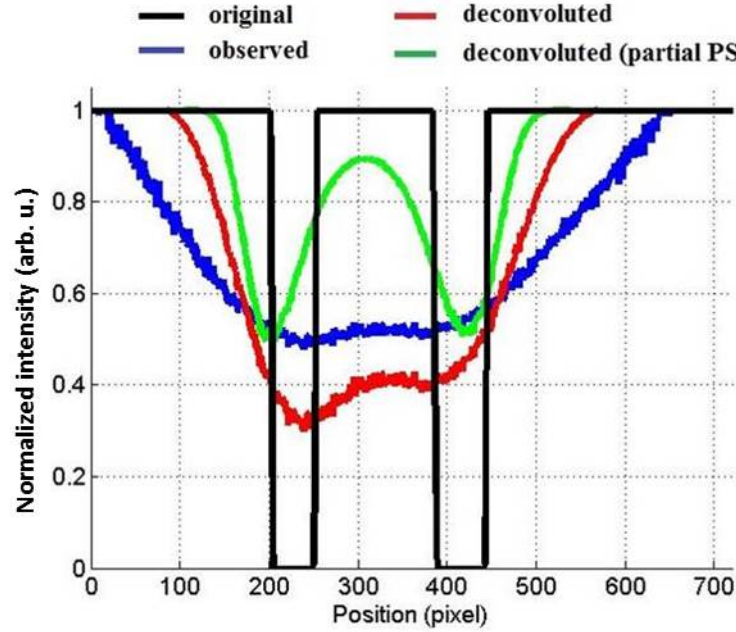
Fig. 4.26. Intensity profiles along the dashed lines in Fig. 4.25.
