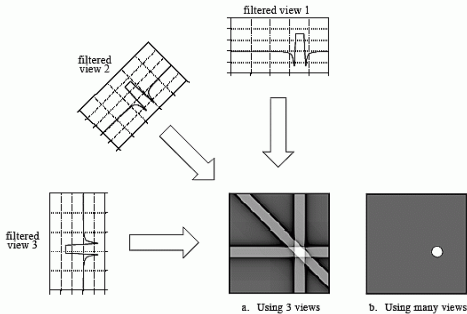
Fig. 3.5. Example of using filtered back-projection technique. Filtered back-projection is reconstructing an image by filtering each view before back-projection. This removes the blurring seen in the simple back-projection as shown in Fig. 3.2, and results in a mathematically exact reconstruction of the image. (Figure reprinted from [3.7])
