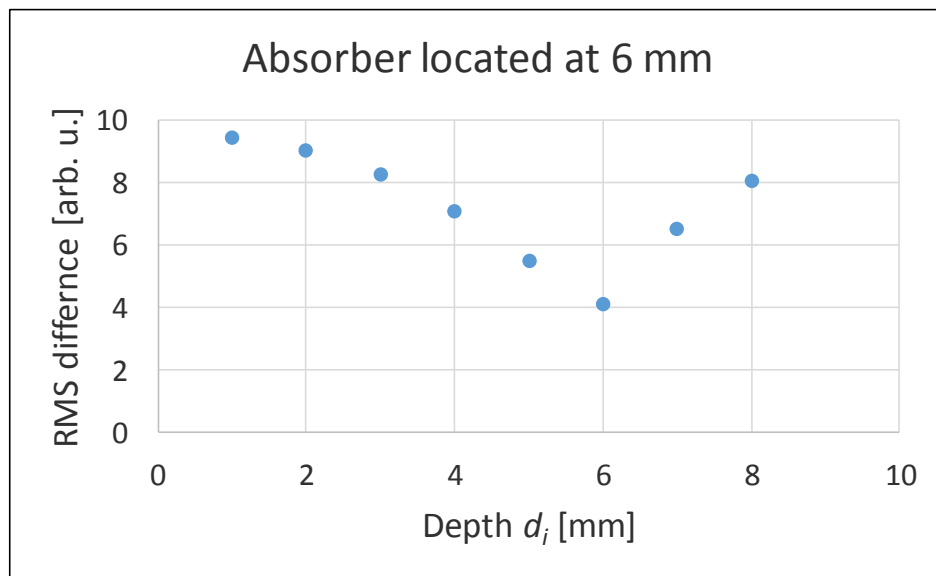
Fig. 8.11. Estimation depth of absorber ( d_t = 6.00 mm).
