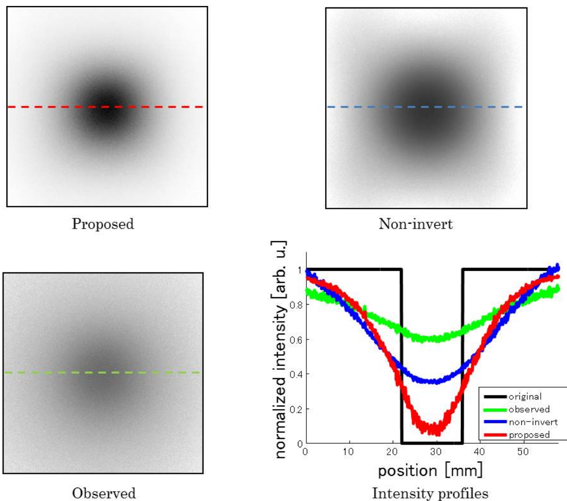
Fig. 4.18. Result with transillumination image of the absorber at d = 10.0 mm. The intensity profiles show the distribution of light intensity along the dashed lines.
