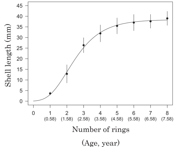
Fig. 4. Growth curve of the short-necked clam, estimated by a Gompertz equation. Plots show mean shell length at each number of rings. Vertical bars show standard deviations of the means.
