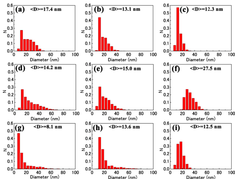
FIG. 3. (a)–(i) Distribution of nanoparticle diameters obtained from the corresponding SEM image in Figs. 2(a)–2(i). N is the proportion of Au nanoparticles.
