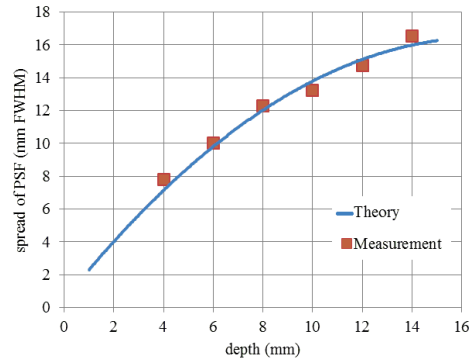
Fig. 4. Comparison between theoretical PSF for light source and measured PSF for absorber.
