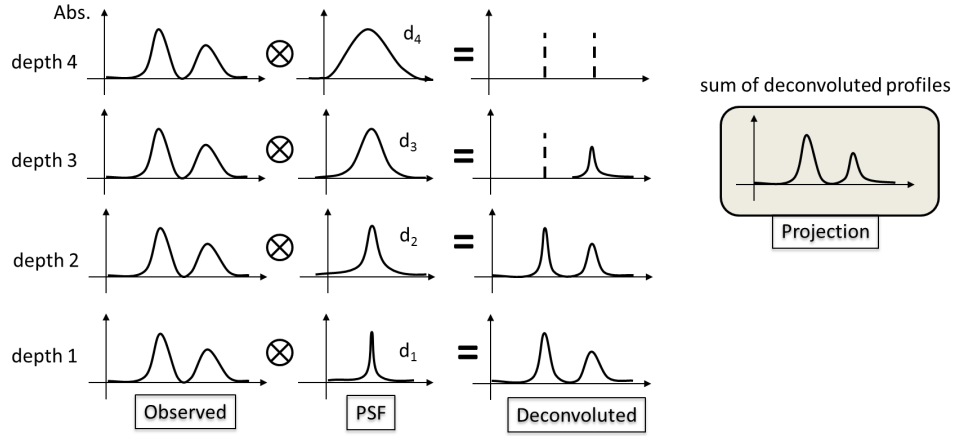
Fig. 16. Absorption profiles before and after the deconvolution with PSFs at different depths. The projection is obtained as a sum of the deconvoluted data with the PSFs at different depths. Profile of projection for cross-sectional reconstruction is shown in upper right corner. \otimes denotes the deconvolution operation.
