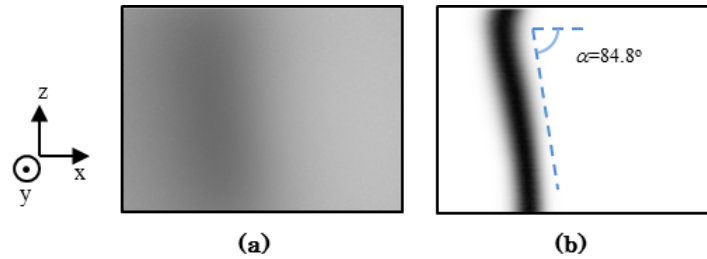
Fig. 9. Observed and deconvoluted images of absorber: (a) observed image (contrast and sharpness are 0.10 and 0.020), (b) deconvoluted image (contrast and sharpness are 0.90 and 0.71).
