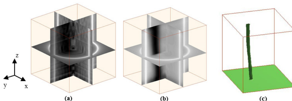
Fig. 14. 3D Reconstruction of absorber in animal tissue: (a) from observed images, (b) from deconvoluted images, (c) result of thresholding on image (b) with a single threshold value.
