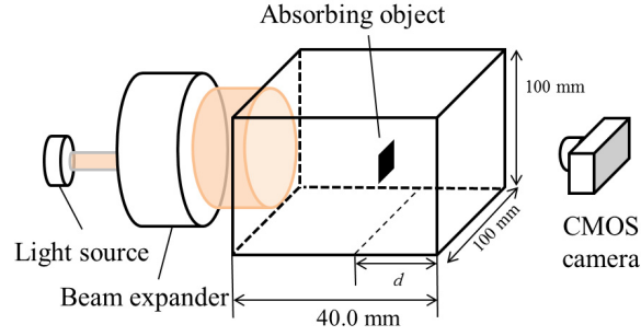
Fig. 2. Experimental setup for transillumination imaging: d = 4.00\text{--}14.0 mm.
