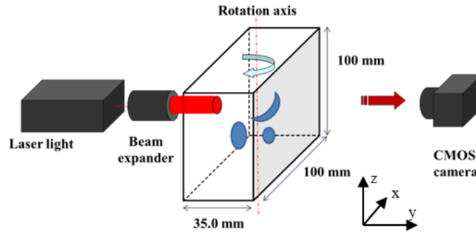
Fig. 19. Experimental setup with phantom.
