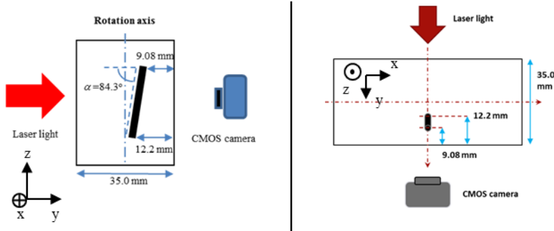
Fig. 8. Side view and top view of phantom model.
