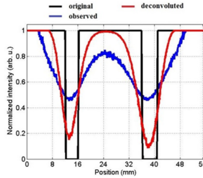
Fig. 6. Intensity profiles along the dashed line in Fig. 5.
