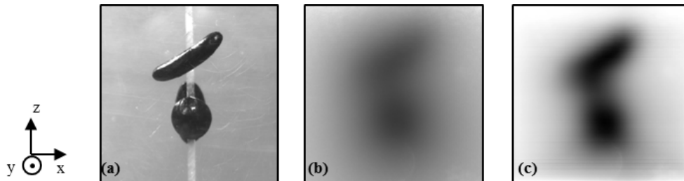
Fig. 20. Scattering suppression in transillumination imaging at 0-deg orientation: (a) observed image in clear medium, (b) observed image in scattering medium, (c) result using the proposed technique.
