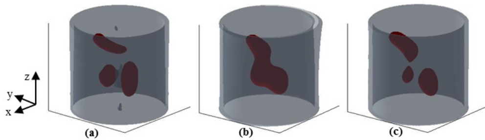
Fig. 22. 3D images reconstructed from transillumination images: (a) from observed image in clear medium, (b) from observed image in scattering medium, (c) result using the proposed technique.
