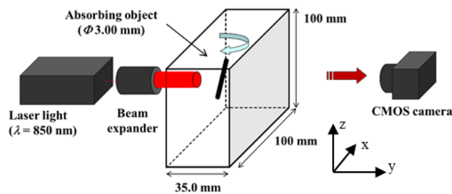
Fig. 7. Experimental setup.
