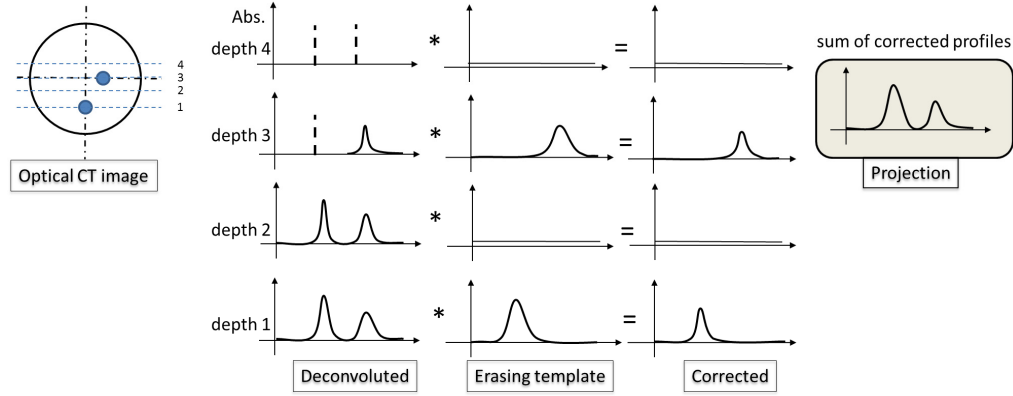
Fig. 17. Principle to suppress erroneous absorption distribution. Erroneous parts are suppressed by multiplying erasing templates obtained from the original cross-sectional image. New projection image is constructed as a sum of the corrected images. * denotes the multiplication operation.
