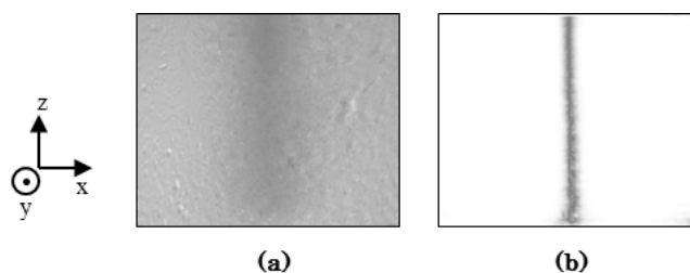
Fig. 13. Observed and deconvoluted images of absorber at 0-deg orientation: (a) observed image (b) result using the proposed technique.
