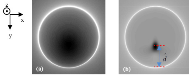
Fig. 11. CT image at the bottom of the absorber: (a) from observed images, (b) from deconvoluted images. Depth of estimated absorber center ( \hat{d} ) was 12.1 mm for true depth 12.2 mm.
