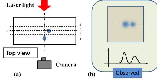
Fig. 15. Two absorbing objects in turbid medium: (a) top view of observing condition, (b) observed transillumination image and absorption profile along the dashed line.
