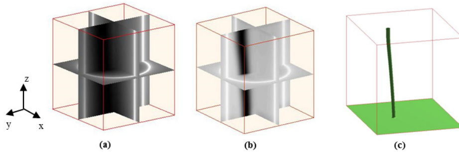
Fig. 12. 3D Reconstruction of absorber in turbid medium: (a) from observed images, (b) from deconvoluted images, (c) result of thresholding on image (b) with a single threshold value.
