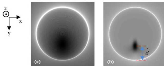
Fig. 10. CT image at the top of the absorber: (a) from observed images, (b) from deconvoluted images. Depth of estimated absorber center ( \hat{d} ) was 9.35 mm for true depth 9.08 mm.
