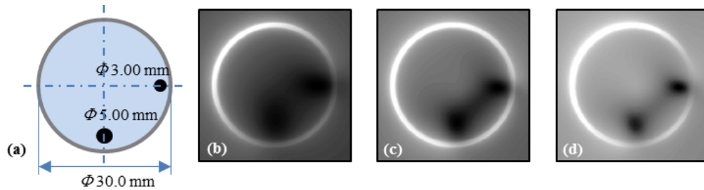
Fig. 18. Result of proposed technique in simulation: (a) simulation model ( \mu'_s = 1.00 /mm, \mu_a = 0.00536 /mm), (b) cross-sectional image of two objects in scattering medium, (c) result from projection of Eq. (3), (d) result from projection of Eq. (4).
