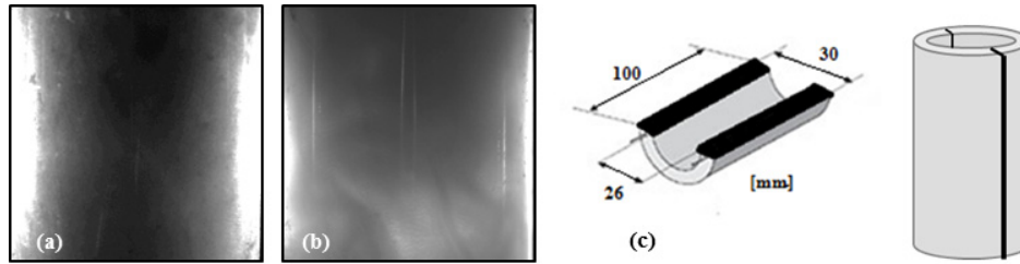
Fig. 24. Suppression of body-surface illumination caused by light-guide effect in cylindrical container: (a) without light trap, (b) with light trap, (c) light trap structure.
