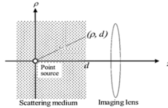
Fig. 1. Geometry for PSF as light distribution observed at the scattering medium surface.
