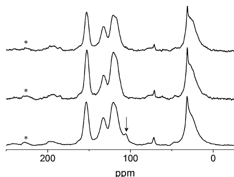
Figure 2. 13 C CP MAS NMR spectra characterizing the RF monoliths treated with 1 N HCl for various periods of time: bottom, no treatment (RFMH-0); middle, 4 days (RFMH-4); top, 20 days (RFMH-20). The arrow indicates a 105 ppm resonance that can be assigned to aromatic carbon between two phenolic carbons. The symbol * indicates a spinning sideband.
