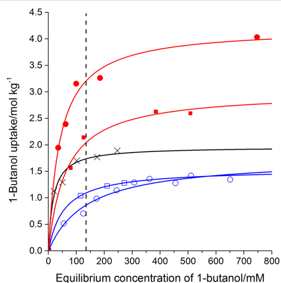
Figure 6. Adsorption isotherms of 1-butanol on CMHs and a high silica MFI zeolite at 310 K: CMH-0-773 (open blue square), CMH-4-773 (solid red square), CMH-0-1073 (open blue circle), CMH-4-1073 (solid red circle), MFI zeolite ( \text{SiO}_2/\text{Al}_2\text{O}_3 = 90 ) (x). The dashed line indicates the upper limit of butanol concentration in biobutanol production.
