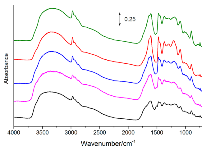
Figure 1. FT-IR spectra characterizing the RF monoliths treated with 1 N HCl for various periods of time: black, no HCl treatment (RFMH-0); magenta, 1 day (RFMH-1); blue, 4 days (RFMH-4); red, 8 days (RFMH-8); green, 20 days (RFMH-20).
