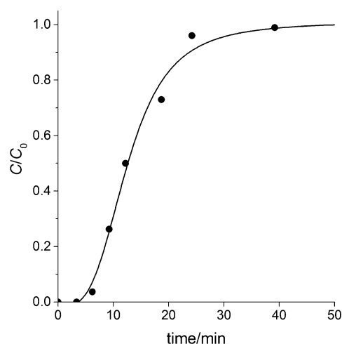
Figure 7. Breakthrough curve of 1-butanol in the CMH-4-1073.
