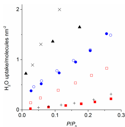
Figure 5. Vapor adsorption of water on pyrolyzed carbons at 298 K: silica gel (x), and MFI zeolite ( \text{SiO}_2/\text{Al}_2\text{O}_3 ratio = 45) (black triangle), coal-derived activated carbon (Norit GAC 1240W) (+), CMH-0-773 (open blue circle), CMH-4-773 (open red square), CMH-0-1073 (solid blue circle), CMH-4-1073 (solid red square).
