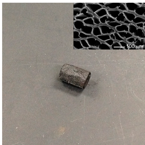
Figure 3. Photograph of a typical CMH synthesized in this work. The inset represents an SEM image of the cross-sectional area of the CMH.
