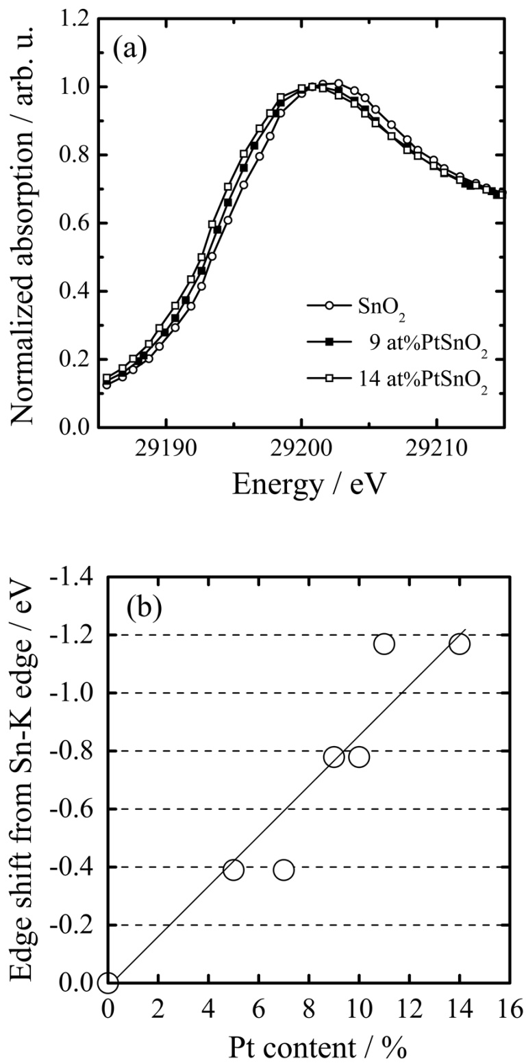
Figure 6. (a) XANES spectra for \text{SnO}_2 , 9 at% and 14 at% Pt/ \text{SnO}_2 , and (b) the Sn K-edge for Pt/ \text{SnO}_2 films with various Pt loading.
