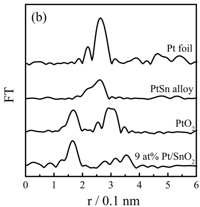
Figure 10. (a) Pt L 3 -edge EXAFS oscillations, and (b) their Fourier transforms. From bottom 9 at % Pt/SnO 2 , PtO 2 , PtSn alloy, Pt-foil.
