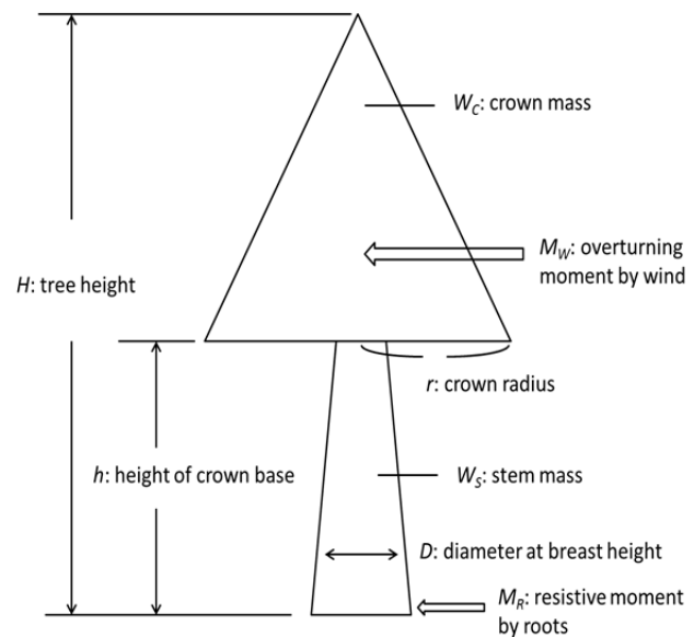
Fig. 1. Abbreviations for tree dimensions and moments.
