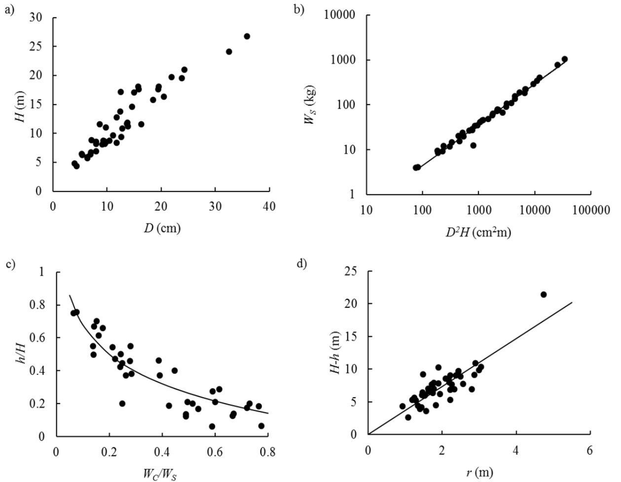
Fig. 2. Relationships among tree size parameters of larch trees (Research Group of Four Japanese Universities 1963). Abbreviations: See Fig.1. Regressions: See Eq. (7) and the text.
