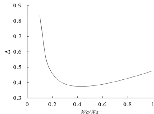
Fig. 3. Change in resistance to uprooting ( \Delta ) with tree shape ( W_C/W_S ). Stem mass is assumed to be 100 kg, and crown mass ranges from 10 to 100 kg. Abbreviations: See Fig. 1.
