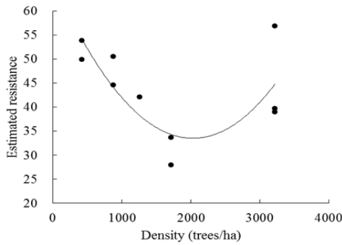
Fig.4. Change in resistance to uprooting of 23-year-old actual Sitka spruce trees (Gardiner et al. 1997), with change in density. Abbreviations: See Fig. 1. Fitted curve: y = 8 \times 10^{-6}x^2 - 0.0032x + 66.4 ( r^2 = 0.57 , p < 0.05 ).
