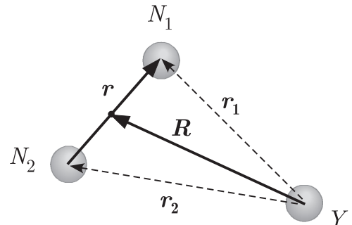
FIG. 4. Coordinates of the 2N - Y systems when calculating the effective 2N - Y potentials.
