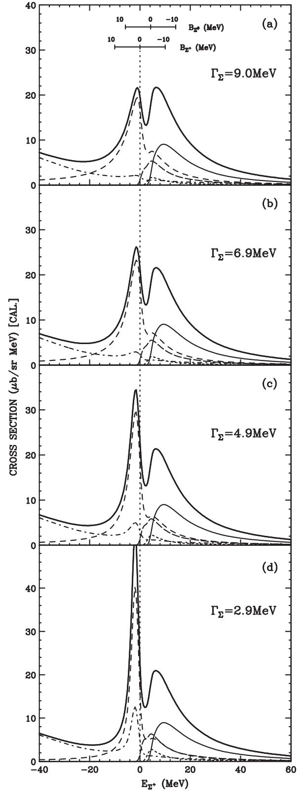
FIG. 12. Shape dependence of the calculated \pi^- spectrum in the {}^3\text{He}(K^-, \pi^-) reaction near the \Sigma threshold at 600 MeV/c ( 4^\circ ), when changing the spreading potential W_{\alpha\alpha'} artificially by f_W = (a) 1.00, (b) 0.75, (c) 0.50, and (d) 0.25, which correspond to widths of \Gamma_\Sigma = 9.0, 6.9, 4.9 , and 2.9 MeV, respectively. These spectra are obtained by folding with a detector resolution of 2 MeV FWHM.
