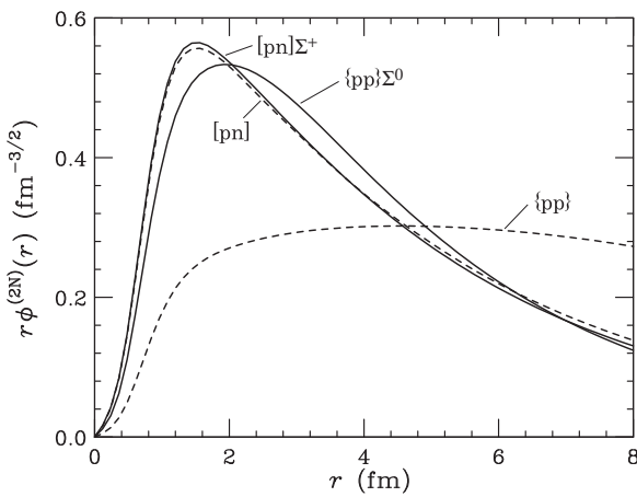
FIG. 5. Radial wave functions of the intranuclear NN states in transition densities of \rho_{\alpha\alpha'} , which are used to calculate the 2N - Y potentials in the folding model, as a function of the relative distance r . The solid curve denote the NN wave functions in the \Sigma NN quasibound state, which is obtained by three-body calculations [18]. The dash curves denote the NN wave functions in free space.
