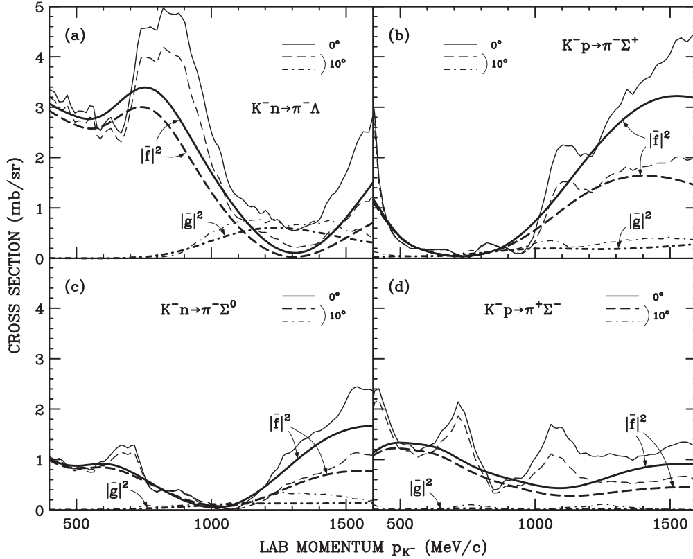
FIG. 3. Fermi-averaged cross sections for (a) K^- + n \rightarrow \pi^- + \Lambda , (b) K^- + p \rightarrow \pi^- + \Sigma^+ , (c) K^- + n \rightarrow \pi^- + \Sigma^0 , and (d) K^- + p \rightarrow \pi^+ + \Sigma^- reactions in nuclear medium. Solid and long-dashed curves denote non-spin-flip Fermi-averaged laboratory cross sections, |\bar{f}|^2 , for \theta_{\text{lab}} = 0^\circ and 10^\circ , respectively, and the dot-dashed curve denotes a spin-flip Fermi-averaged one, |\bar{g}|^2 , for \theta_{\text{lab}} = 10^\circ . The thin-solid and thin-dashed curves are for non-spin-flip laboratory elementary cross sections in free space at \theta_{\text{lab}} = 0^\circ and 10^\circ , respectively, and the thin-dot-dashed curve is for a spin-flip one at \theta_{\text{lab}} = 10^\circ . The elementary amplitudes are used by Gopal et al. [49].
