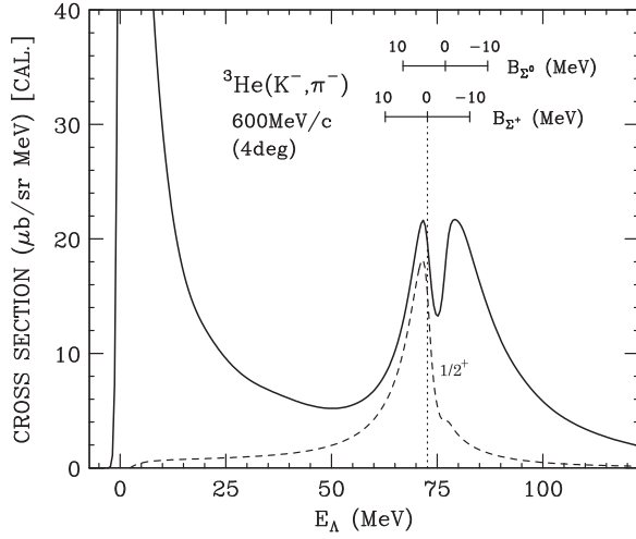
FIG. 7. Calculated inclusive \pi^- spectrum of the ^3\text{He}(K^-, \pi^-) reaction at 600 MeV/c ( 4^\circ ). The solid curve denotes the total spectrum, and the dashed curve denotes the J^\pi = 1/2^+ ( L=0 , S=1/2 ) component caused by conversion decay processes as [\Sigma^3\text{He}] \rightarrow p + p + \Lambda , with a detector resolution of 2 MeV FWHM.
