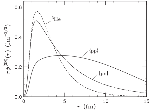
FIG. 2. Behaviors of the radial wave functions of the NN states, r\phi^{(2N)}(r) , as a function of the relative distance r between the nucleons. The solid and long-dashed-dot curves denote the wave functions for \{pp\} and [pn] , respectively. The dashed curve denotes the intranuclear NN wave function in the {}^3\text{He} ground state, which is obtained by three-body calculations. All of the wave functions are calculated with the central Tamagaki's C3G potential [32].
