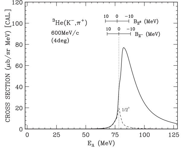
FIG. 9. Calculated inclusive \pi^+ spectrum of the ^3\text{He}(K^-, \pi^+) reaction at 600 MeV/c ( 4^\circ ). The solid curve denotes the total spectrum, and the dashed curve denotes the J^\pi = 1/2^+ ( L=0 , S=1/2 ) component caused by conversion decay processes as [\Sigma^3n] \rightarrow n + n + \Lambda , with a detector resolution of 2 MeV FWHM.
