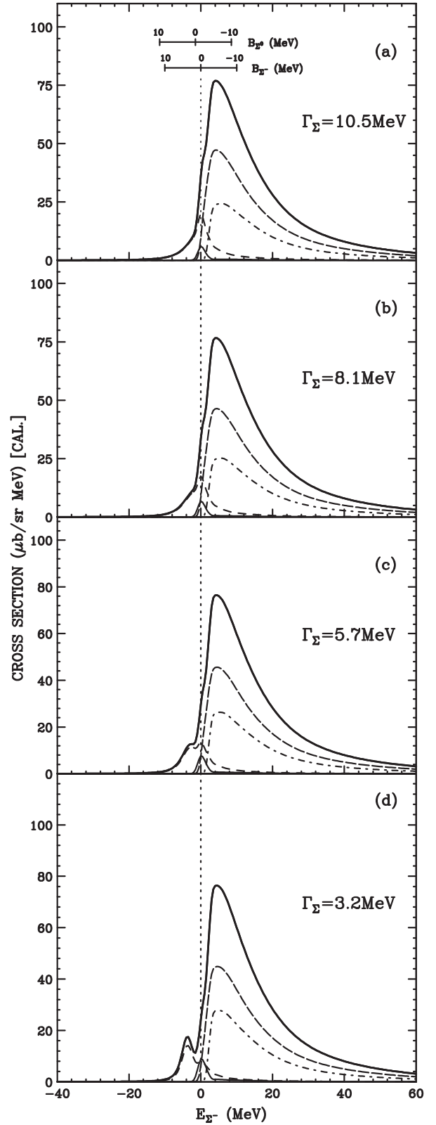
FIG. 13. Shape dependence of the calculated \pi^+ spectrum in the {}^3\text{He}(K^-, \pi^+) reaction near the \Sigma threshold at 600 MeV/c ( 4^\circ ), when changing the spreading potential W_{\alpha\alpha'} artificially by f_W = (a) 1.00, (b) 0.75, (c) 0.50, and (d) 0.25, which correspond to widths of \Gamma_\Sigma = 10.5, 8.1, 5.7 , and 3.2 MeV, respectively. These spectra are obtained by folding with a detector resolution of 2 MeV FWHM.
