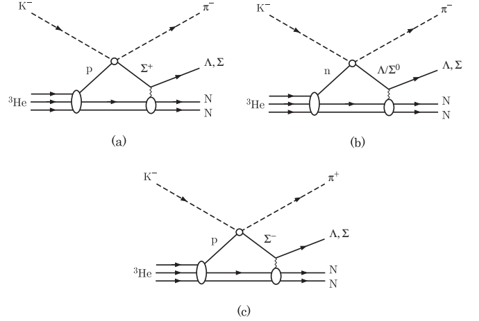
FIG. 1. Diagrams for hypernuclear (K^-, \pi^\mp) reactions on a {}^3\text{He} target: (a) K^- + p \rightarrow \pi^- + \Sigma^+ , (b) K^- + n \rightarrow \pi^- + \Lambda or K^- + n \rightarrow \pi^- + \Sigma^0 , and (c) K^- + p \rightarrow \pi^+ + \Sigma^- reactions in the impulse approximation.
