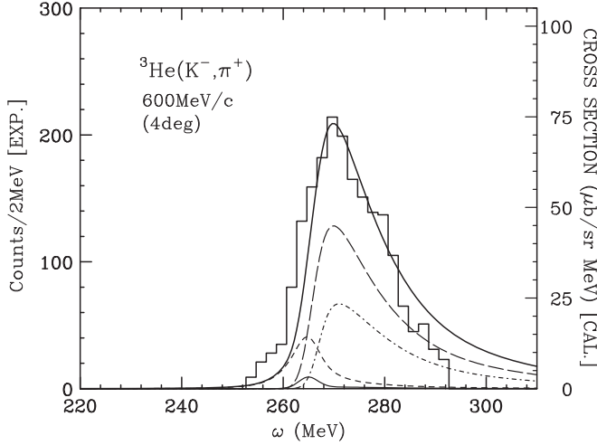
FIG. 14. Comparison of the calculated \pi^+ spectrum with the experimental data in the {}^3\text{He}(K^-, \pi^+) reaction at 600 MeV/c ( 4^\circ ). The bold solid curve denotes the inclusive \pi^+ spectrum obtained by folding with a detector resolution of 5 MeV FWHM. The dashed, long-dashed, dot-dashed, and thin-solid curves denote the contribution of the [\frac{3}{2}n] \rightarrow n + n + \Lambda decay, [pn]\Sigma^- , \{pn\}\Sigma^- , and \{nn\}\Sigma^0 components, respectively. Data are taken from BNL-E774 [20].
