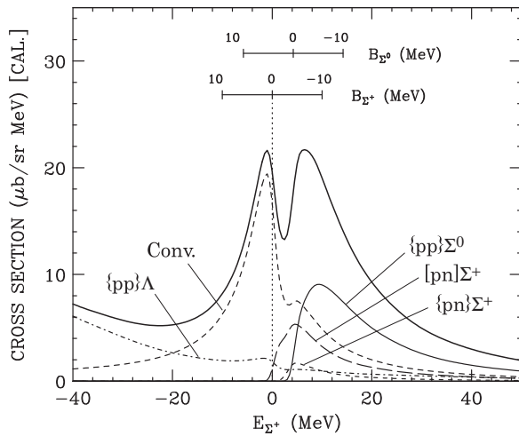
FIG. 8. The decomposition of the calculated inclusive \pi^- spectrum of the ^3\text{He}(K^-, \pi^-) reaction at 600 MeV/c ( 4^\circ ) near the \Sigma threshold, together with the components of \{pp\}\Lambda , [pn]\Sigma^+ , \{pn\}\Sigma^+ , \{pp\}\Sigma^0 , and [\Sigma^3\text{He}] \rightarrow p + p + \Lambda conversion processes, obtained by folding with a detector resolution of 2 MeV FWHM.
