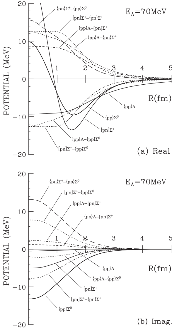
FIG. 6. (a) Real and (b) imaginary parts of the calculated effective 2N - Y potential \hat{U}_{\alpha\alpha'}(R) for {}^3_2\text{He} ( J^\pi = 1/2^+ ) at E_\Lambda = 70 MeV in the folding-model potential, as a function of a relative distance R between 2N and Y .
