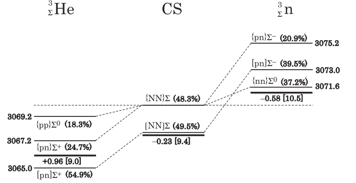
FIG. 11. Energies and widths of the \Sigma NN quasibound states (thick line) near the \Sigma threshold. The square brackets denote the widths of the quasibound states, and the round brackets denote probabilities of each channel component. See also Tables IV and V.
