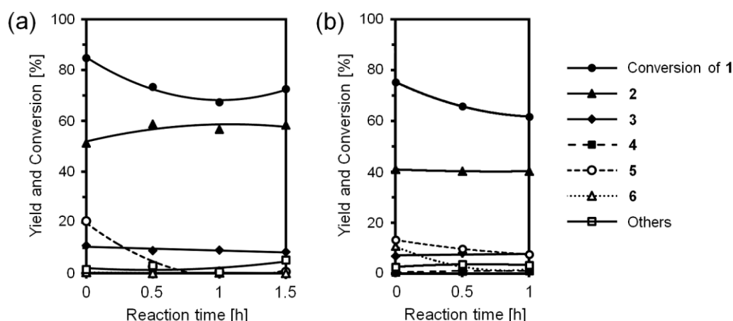
Fig. 7 Time-course of the HDO of 4-propylphenol 1 at 300 °C by (a) Pt-Re/ZrO 2 and (b) Pt/ZrO 2 . Reaction conditions: see entries 1 and 2 in Table 2.
