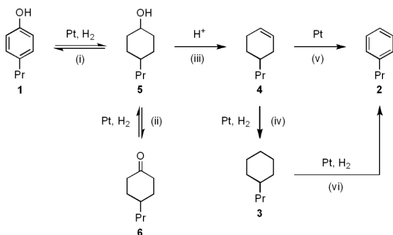
Fig. 8 Proposed reaction pathways.
