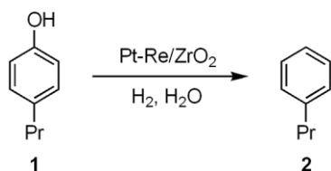
Scheme 1 Selective conversion of 4-propylphenol 1 to n -propylbenzene 2 .
