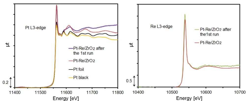
Fig. 4 Pt L 3 -edge and Re L 3 -edge XANES spectra of Pt-Re/ZrO 2 catalysts.
