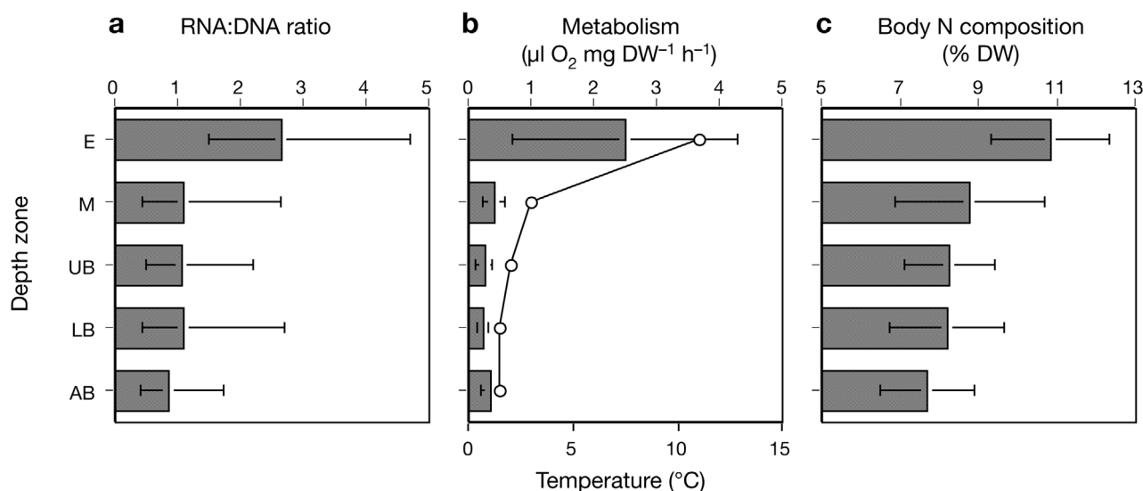
Fig. 3. Depth-related decline in (a) RNA:DNA ratios (this study), (b) metabolism (bar) vs. temperature (O) (Ikeda et al. 2006a), and (c) body N content (Ikeda et al. 2006b) of pelagic copepods (see Table 2 for depth-zone abbreviations) in the North Pacific. Data are means ( \pm SD). To make direct comparison with RNA:DNA ratios of this study possible, we replaced metabolism and body N content data of epipelagic copepods from Ikeda et al. (2006a,b) (Arctic/Antarctic copepods) with those of epipelagic copepods in the North Pacific (i.e. data from the appendix of Ikeda et al. 2007); this change did not alter the overall depth-related reduction patterns of metabolism and body N content appreciably. The temperature of each depth zone was represented by those adopted as in situ temperatures for respiration (metabolism) experiments (cf. Ikeda et al. 2007)
