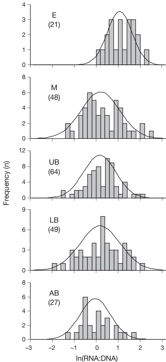
Fig. 2. Log-transformed RNA:DNA ratios of copepods (see Table 2 for depth-zone abbreviations) in the North Pacific. Values in parentheses: number of datasets. Normalized data were used for the calculation of means, SDs and statistical comparisons (see Tables 2 & 3)
