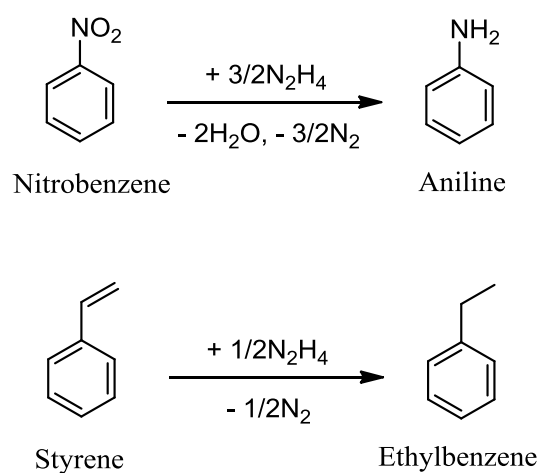
Scheme 1. Reduction of nitrobenzene and styrene by hydrazine
