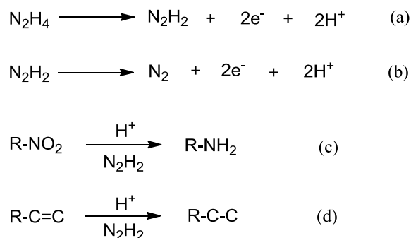
Scheme 3. Possible pathways for the reduction of nitro and vinyl groups by hydrazine [8, 12, 14]
