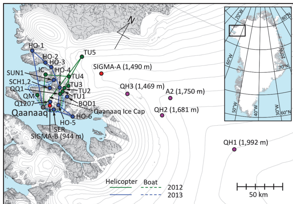
Fig. 4. Map showing the location of observation sites in the Qaanaaq area of northwest Greenland. The contour interval is 100 m. Red and pink colored circles indicate AWS stations established in 2012 and glaciological/meteorological observation sites, respectively, and the elevations are given in the parentheses. These sites were accessed by helicopter. Green and blue colored circles indicate biological observation sites in 2012 and 2013, respectively. Solid and dashed lines connected with those circles indicate the helicopter and boat routes, respectively, in each year.
