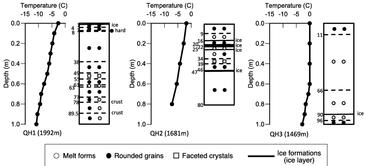
Fig. 5. Snow stratigraphy and vertical profiles of snow temperature in snow pits at sites QH1, QH2 and QH3 on July 30, 2011. The characters showing snow classification are in accordance with the snow classification by Fierz et al. (2009), which are indicated in the legend.
