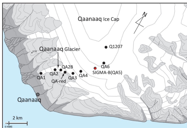
Fig. 2. Map showing the location of observation sites on the Qaanaaq Ice Cap. The contour interval is 100 m and the contour lines higher than 700 m do not agree with the site elevations measured with GPS as shown in Tables 1–3. The red colored circle is an AWS station.
