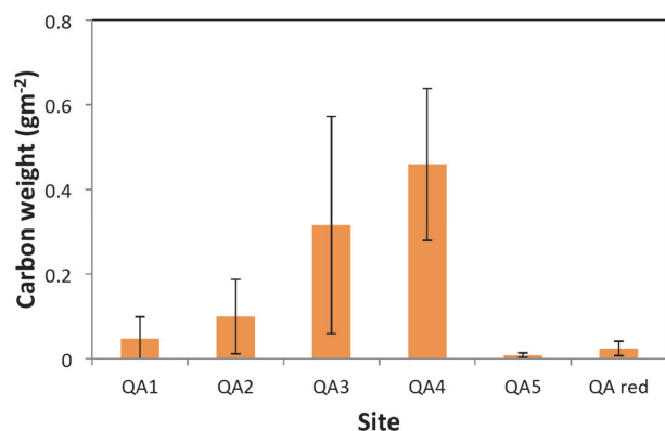
Fig. 14. Amounts of carbon weight ( \text{g m}^{-2} ) of large cryoconite (more than 250 mm in diameter) from QA1 to QA5 and QA-red.
