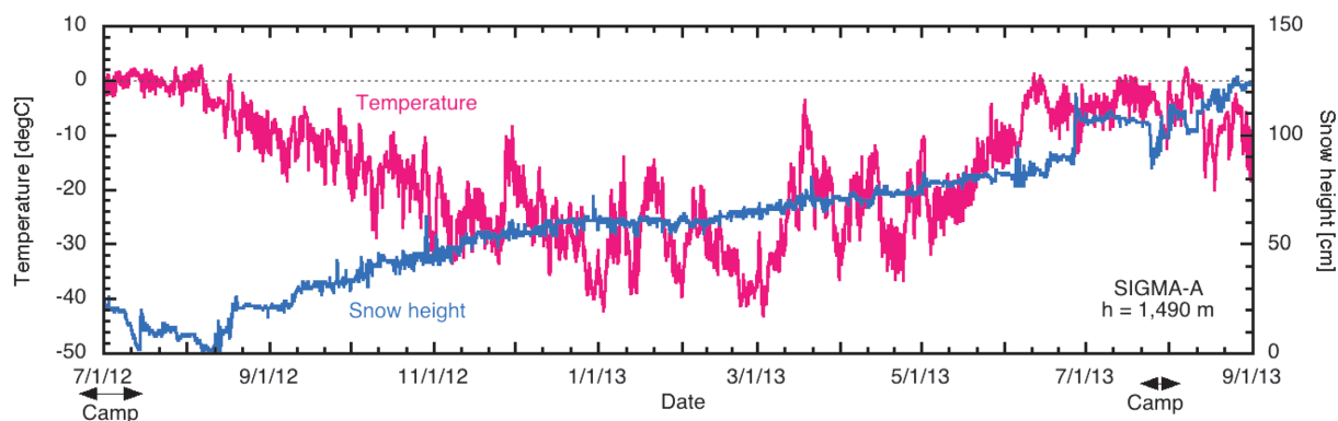
Fig. 9. Time series variation of air temperature at a height of 3 m and snow height measured with an AWS at SIGMA-A from July 2012 to August 2013. Snow height is a relative value to the minimum in the summer of 2011.
