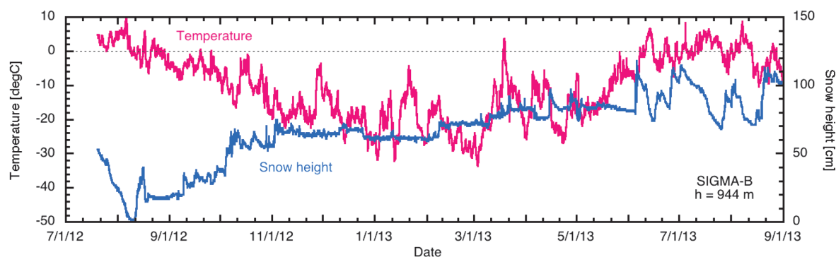
Fig. 13. Time series variation in air temperature at a height of 3m and snow height measured with AWS at SIGMA-B from July 2012 to August 2013. Snow height is a relative value to the minimum in the summer of 2011.
