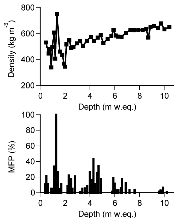
Fig. 11. Profiles of the bulk density (top) and melt feature percentage (MFP) in a 0.1 m long section (bottom) of the firn-ice core obtained from SIGMA-A on July 3 and 6, 2012.
