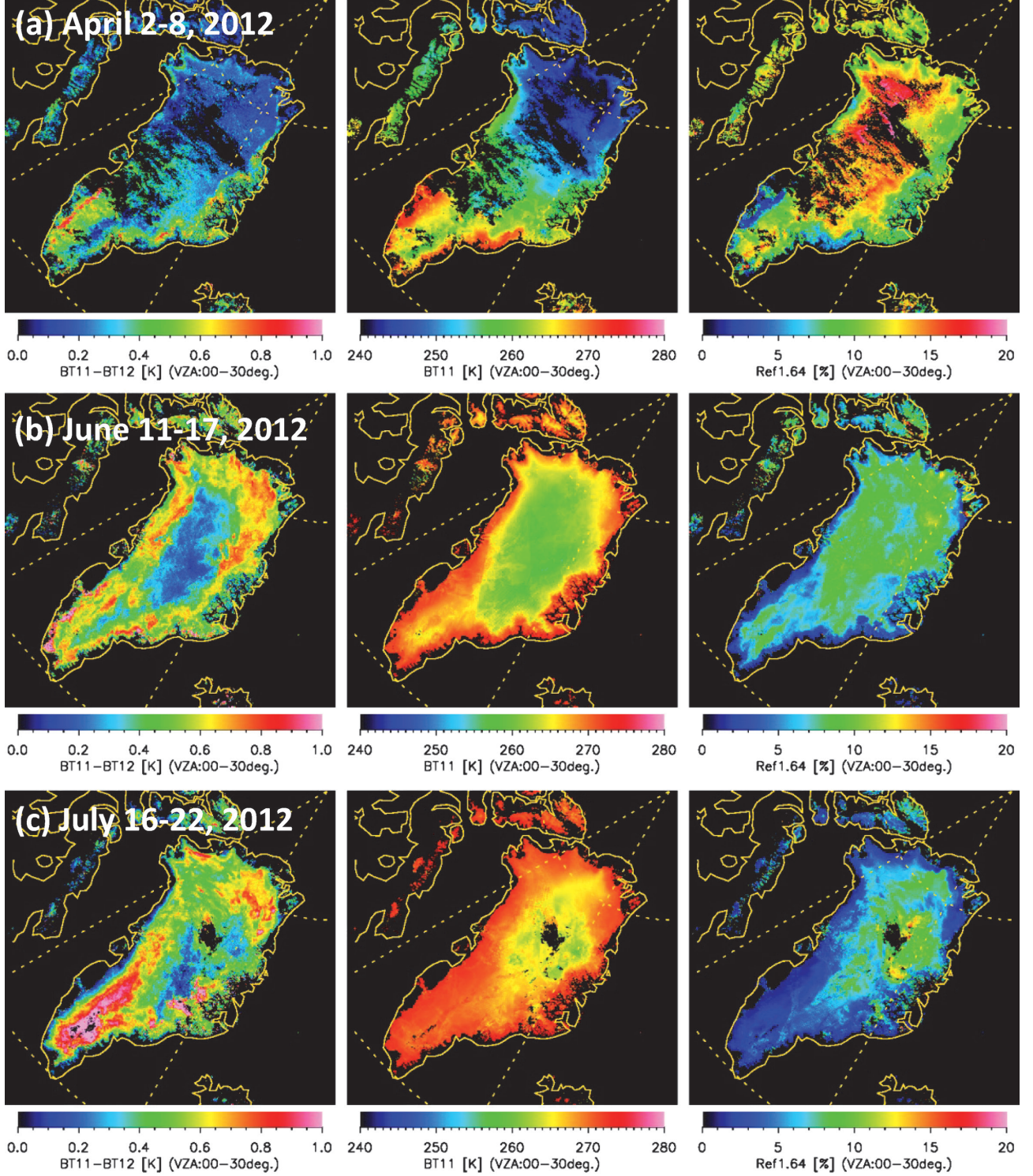
Fig. 7. Spatial distribution of brightness temperature difference ( BTD_{sat} ) between 11 \mu\text{m} and 12 \mu\text{m} (left), brightness temperature at \lambda = 11 \mu\text{m} ( BT11_{sat} ) (middle) and reflectance at \lambda = 1.6 \mu\text{m} ( Ref1.6_{sat} ) (right) observed over the Greenland ice sheet in the period of (a) 2-8 April, (b) 11-17 June and (c) 16-22 July 2012. The black color over the ice sheet denotes remaining cloudy areas that could not be eliminated in the weekly composite period.
