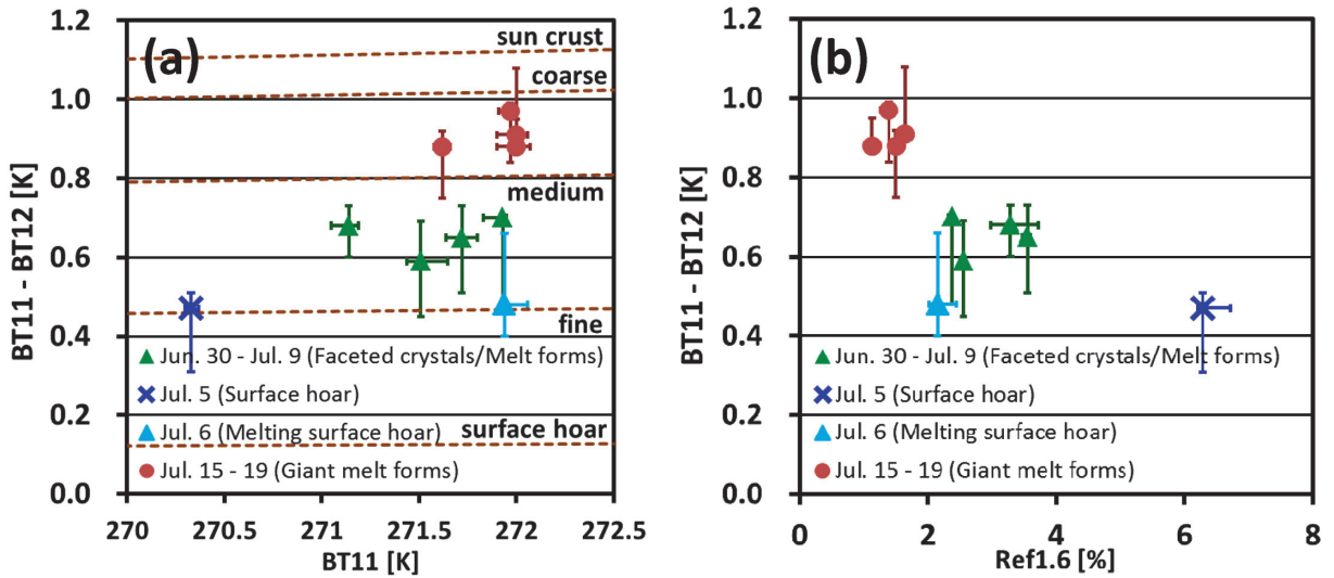
Fig. 6. Scatter plots of (a) Brightness temperature at \lambda = 11 \mu\text{m} ( \text{BT}11_{\text{sat}} ) and brightness temperature difference between 11 \mu\text{m} and 12 \mu\text{m} ( \text{BTD}_{\text{sat}} = \text{BT}11_{\text{sat}} - \text{BT}12_{\text{sat}} ) and (b) reflectance at \lambda = 1.6 \mu\text{m} ( \text{Refl.}1.6_{\text{sat}} ) and \text{BTD}_{\text{sat}} extracted from the center pixel of the match-up image in Fig. 4. Error bars denote the maximum and minimum values within the surrounding eight pixels. Also plotted in the left figure are the expected \text{BTD} lines, which are averages of the simulated \text{BTD}_{\text{sim}} at near-nadir satellite zenith angles between 0 and 30^{\circ} shown in Fig. 3.
