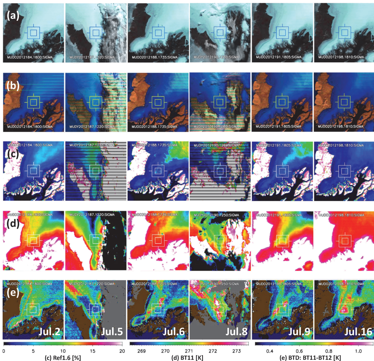
Fig. 4. Match-up analysis images of (a) MODIS true-color RGB composite, (b) false-color RGB composite, (c) reflectance at the wavelength ( \lambda ) of 1.6 \mu\text{m} ( Ref1.6_{sat} ), (d) brightness temperature at \lambda=11 \mu\text{m} ( BT11_{sat} ) and (e) brightness temperature difference between MODIS channels 31 and 32 ( BTD_{sat}=BT11_{sat}-BT12_{sat} ) observed at the SIGMA-A site during the in situ observation period (2, 5, 6, 8, 9 and 16 July 2012). The SIGMA-A site is located at the center of these images within the box. Color legends for Fig. 4 (c), (d) and (e) are shown at the bottom. In Fig. 4 (e), gray, brown and blue colors denote clouds, bare land and open ocean, respectively.
