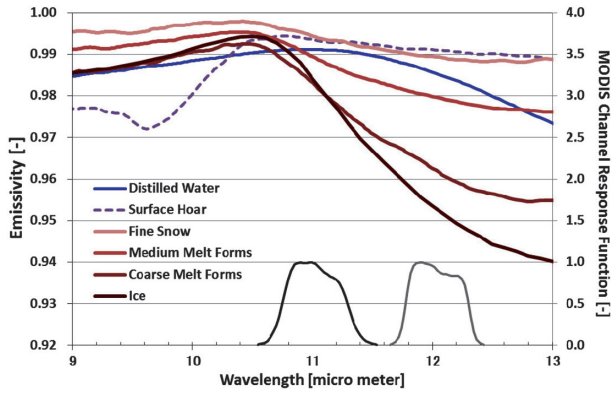
Fig. 1. Spectral directional emissivity of various surface types in the thermal infrared window region (exitance angle is 10^\circ from the normal) all taken from the ASTER spectral library (1999). Also plotted are response functions of MODIS TIR channels at \lambda = 11.0 \mu\text{m} and 12.0 \mu\text{m} . Snow types are employed according to the international classification of snow crystals (Fierz et al. , 2009).
