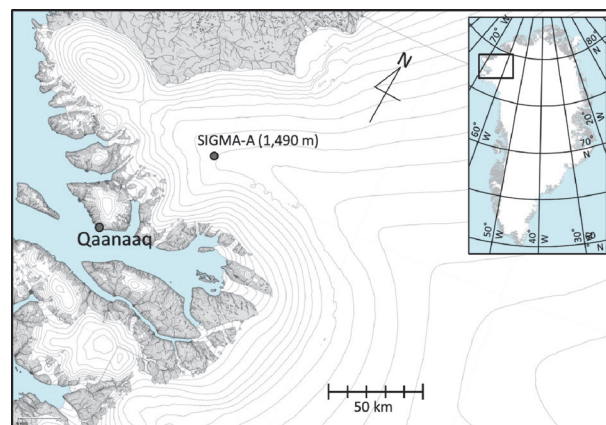
Fig. 2. Location of in situ observation site at the northwestern part of the Greenland ice sheet (SIGMA-A site: 78^\circ03'06''\text{N} , 67^\circ37'42''\text{W} , 1490 m a.s.l.).
