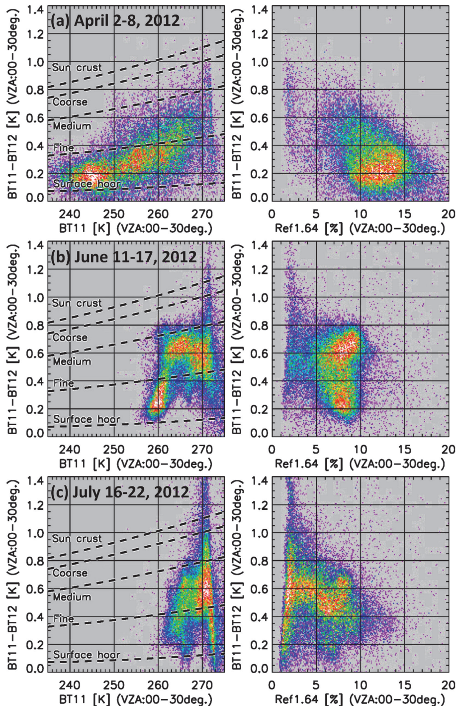
Fig. 8. Scatter plot between BT11_{sat} and BT12_{sat} (left column) and Ref1.6_{sat} and BT12_{sat} (right column) extracted from the images shown in Fig. 7 in the period of (a) 2–8 April, (b) 11–17 June and (c) 16–22 July 2012. Also plotted in the left column figures are the expected BTD lines for the snow types of surface hoar, fine snow, medium melt forms, coarse melt forms and sun crust, which are averages of the simulated BTD_{sim} at near-nadir satellite zenith angles between 0–30° shown in Fig. 3.
