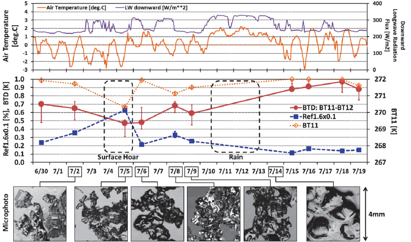
Fig. 5. (Upper) Temporal series of air temperature ( ^{\circ}\text{C} ) and downward longwave radiation flux ( \text{W}/\text{m}^2 ) measured with the automatic weather station at the SIGMA-A site during 30 June to 19 July 2012. (Middle) Temporal variations of satellite-derived reflectance at \lambda = 1.6 \mu\text{m} ( \text{Refl.}1.6_{\text{sat}} in %, the value of which is multiplied by 0.1), brightness temperature at \lambda = 11 \mu\text{m} ( \text{BT}11_{\text{sat}} in Kelvin) and brightness temperature difference between 11 \mu\text{m} and 12 \mu\text{m} ( \text{BTD}_{\text{sat}} in Kelvin) extracted at the center pixel of the MUD images shown in Fig. 4. Error bars denote the maximum and minimum values within the surrounding eight pixels. (Lower) Micro-photos of surface snow crystals taken at the site.
