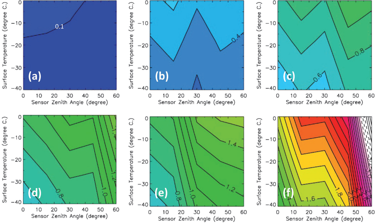
Fig. 3. Simulated brightness temperature differences ( BTD_{sim} ) between MODIS channels 31 ( \lambda = 11 \mu\text{m} ) and 32 ( \lambda = 12 \mu\text{m} ) at the top of the atmosphere as functions of satellite zenith angle and surface temperature calculated using spectral emissivities for the various snow and water surfaces of (a) surface hoar, (b) fine snow, (c) medium melt forms, (d) coarse melt forms, (e) sun crust and (f) bare specular ice.
