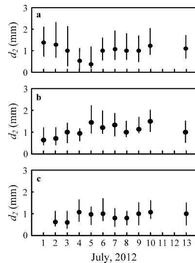
Fig. 8. Measurement results of d_2 near the surface in 2012. Black circles indicate the medium values at each measurement position. Bars indicate the range of d_2 from maximum to minimum. a. Data at 0–2 cm depth from the surface. b. Data at 2–5 cm depth from the surface. c. Data at 5–10 cm depth from the surface.
