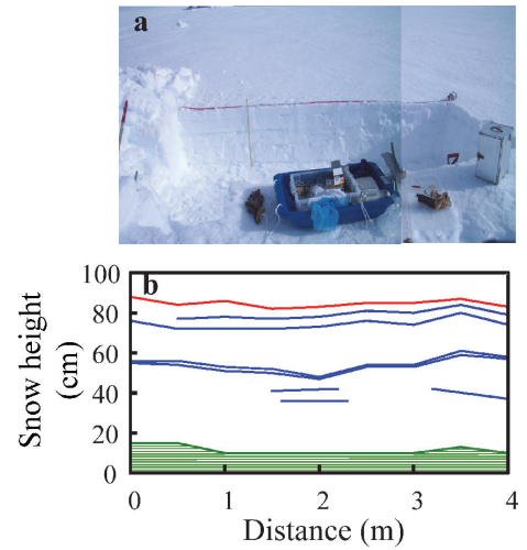
Fig. 7. Measurement results of 4 m wide snow pit on July 4, 2012.
