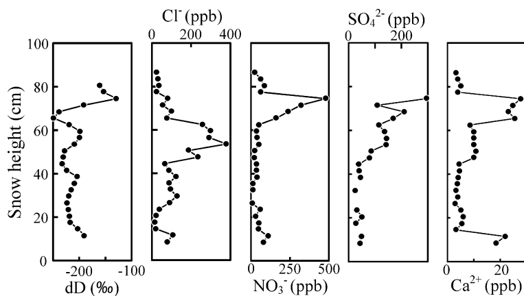
Fig. 10. Results of chemical analyses of snow samples obtained on June 30, 2012.
