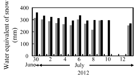
Fig. 6. Measurement results of the water equivalent of snow cover in 2012.
