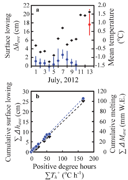
Fig. 3. Results of snow-stake observations in 2012.
