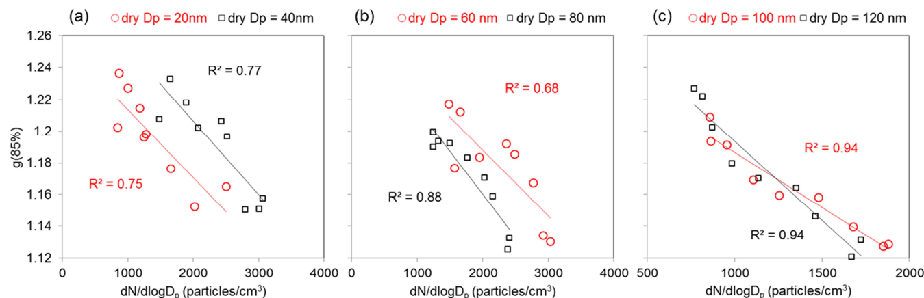
Figure 5. Scatter plots of g(85\%) versus particle number concentrations in each size bin during the NPF events. (a) Dry D_p = 20 and 40 nm. (b) Dry D_p = 60 and 80 nm. (c) Dry D_p = 100 and 120 nm. The data points are 30 min averaged g(85\%) values and particle number concentrations from 04:00 to 08:00 LT are marked (A) in Fig. 4a and c.
