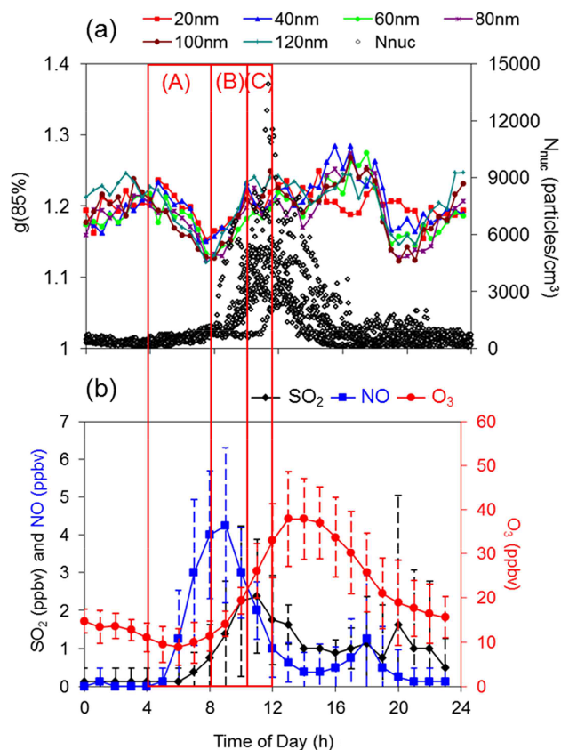
Figure 4. Diel variations in (a) median g(85\%) values in the dry D_p range of 20–120 nm with a 20 nm increment and N_{nuc} , and (b) SO_2 , NO , and O_3 concentrations during the NPF events. g(85\%) at dry D_p = 20 , 40, 60, and 80 nm were converted to equivalent g(85\%) of dry D_p = 100 nm by considering the Kelvin effect. Error bars in (b) represent standard deviations ( 1\sigma ) of SO_2 , NO , and O_3 concentrations.
