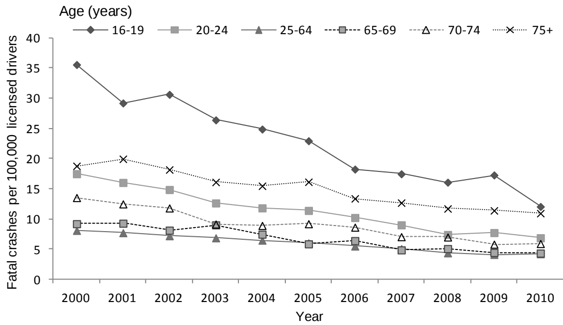
Figure A1 Fatal four-wheeled motor vehicle crashes per 100,000 licensed drivers among primary party* by age group in Japan, 2000–2010
