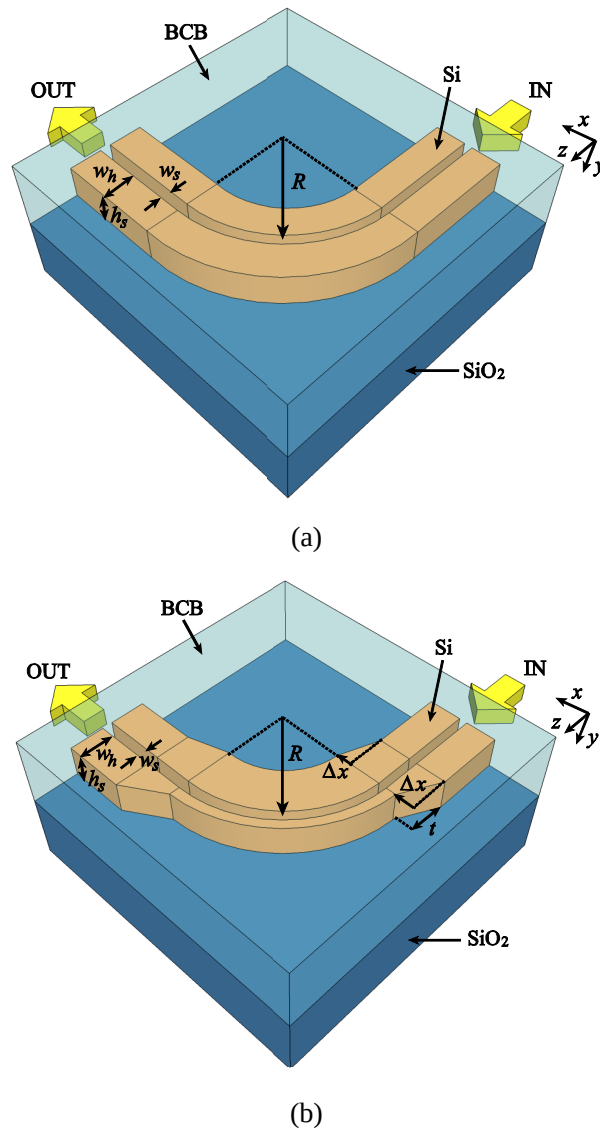
Fig. 5.1: Schematics of (a) a conventional silicon slot waveguide bend and (b) a silicon slot waveguide bend with an asymmetric slot.
