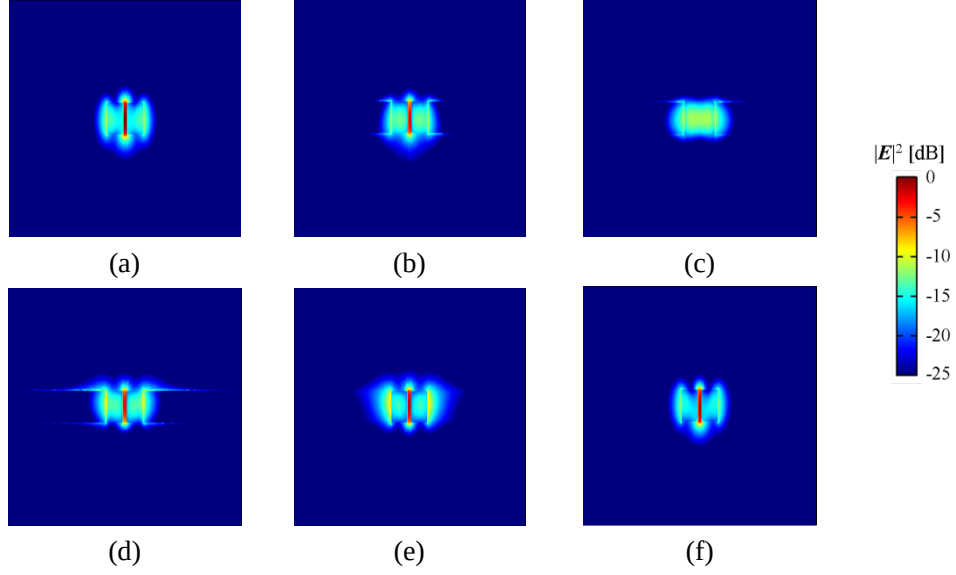
Fig. 4.5: The electric field intensity distributions on the x-y plane in several z-positions at \lambda = 1.55 \mu\text{m} . Each of (a)-(f) corresponds to the z coordinates of A-F in Fig. 2(c), respectively.
