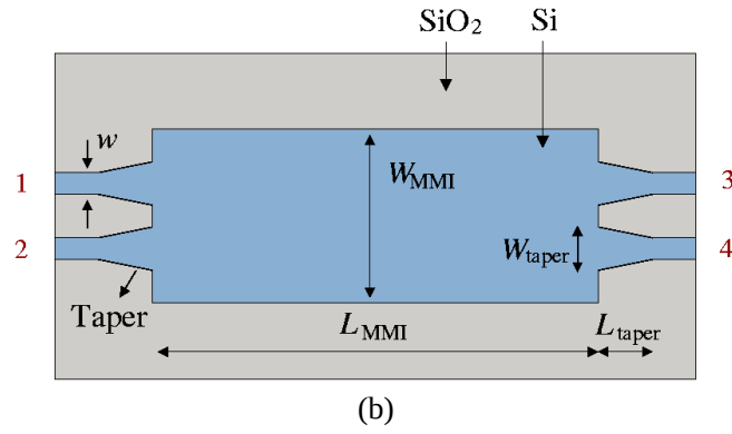
Fig. 3.2: (a) Schematic of optical XOR, XNOR, NAND and OR logic gates. (b) Structure of the MMI-based 3-dB coupler.
