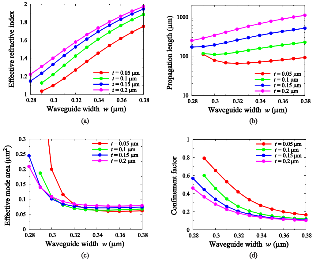
Fig. 6.4: (a) The effective refractive index, (b) the propagation length, (c) the effective mode area, and (d) the confinement factor as a function of the waveguide width w when h = 0.22 \mu\text{m} .
