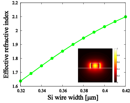
Fig. 5.6: The effective refractive index of the Si wire waveguide as a function of the width of the Si wire when h = 0.2 \mu\text{m} .
